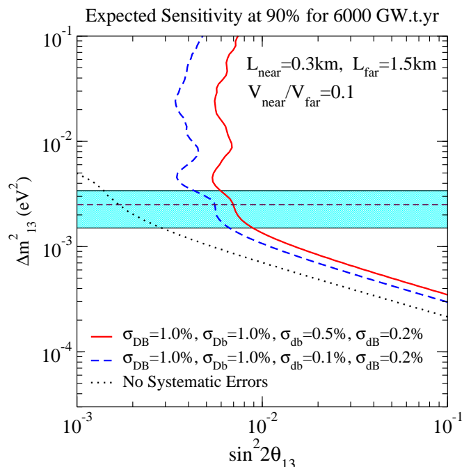
FIG. 6: 90% CL sensitivity curve in the parameter space of \Delta m_{13}^2 and \sin^2 2\theta_{13} for 3 years of data taking assuming the same systematic errors as in Fig. 5. The blue band indicates the allowed range of \Delta m_{13}^2 coming from atmospheric neutrino observation [11].
