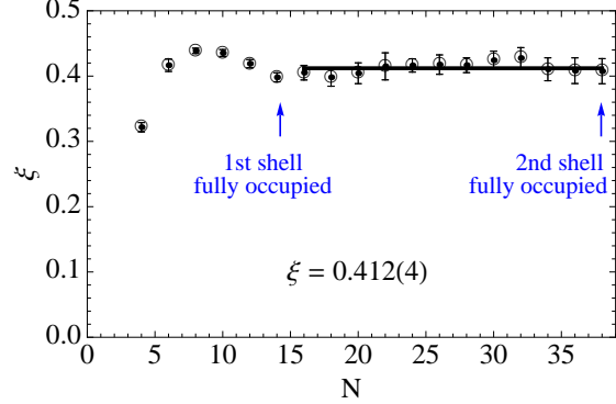
Figure 4: (Preliminary) Bertsch parameter as a function of N for V = 12^3 . The solid line represents the fitting range and fit result for \xi .
