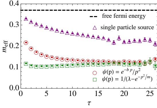
Figure 1: Effective mass plots for L = 8 , M = 5 , and N = 8 ( N_\uparrow = N_\downarrow = 4 ). The purple triangles are obtained using the lowest momentum eigenstates for an uncorrelated single free fermion while red circles and green squares are obtained using correlated two-particle states for spin up and down as sinks. The black dashed line correspond to the ground state energy for non-interacting fermions. b = 0.5 and \lambda = 1.01 are used for red and green, respectively.
