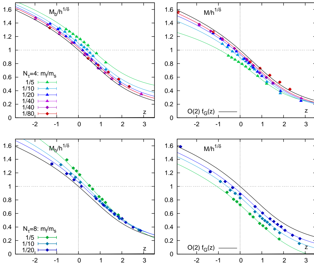
FIG. 1. Fit of the O(2) scaling function to numerical results for the subtracted order parameter M (right) and the non-subtracted light quark condensate M_b (left), both for N_\tau = 4 (top) and N_\tau = 8 (bottom). The fits include an ansatz for violations of scaling as discussed in the text. Shown are results for m_l/m_s \leq 1/5 .
