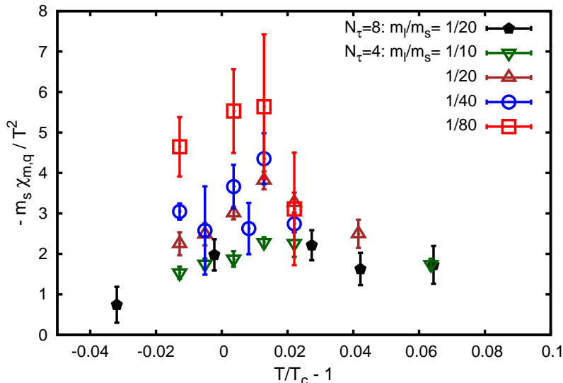
FIG. 2. The mixed light quark number susceptibility as a function of the reduced temperature, (T - T_c)/T_c . Shown are results obtained at two values of the cut-off, N_\tau = 4 (open symbols) and N_\tau = 8 (filled symbols), and for several values of the light to strange quark mass ratio.
