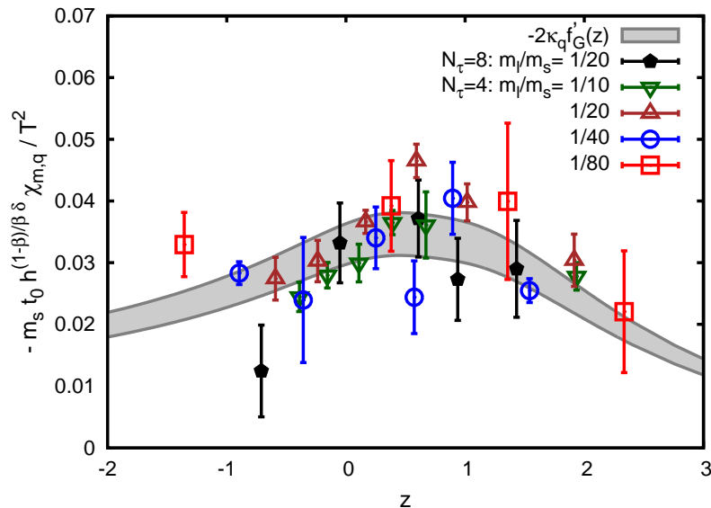
FIG. 3. The scaled mixed susceptibility as function of the scaling variable z = t/h^{1/\beta\delta} . The data are compared to the O(2) scaling curve. The band shows a 10% error band on this curve which arises from statistical errors on the calculated observables as well as from the errors on the scaling parameters t_0 and z_0 given in Table I.
