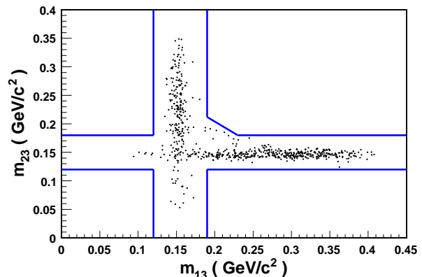
FIG. 6: Distribution of m_{13}-m_{23} of the data with all selection cuts imposed. No event was observed in the signal region.
