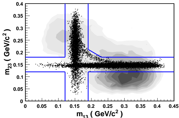
FIG. 3: Distribution of m_{13} - m_{23} of the MC events with three clusters in the CsI calorimeter. The contour shows the K_L^0 \rightarrow 3\gamma parity-violating results, and the dots show the K_L^0 \rightarrow \pi^0\pi^0 results. The events inside the cross region were rejected.
