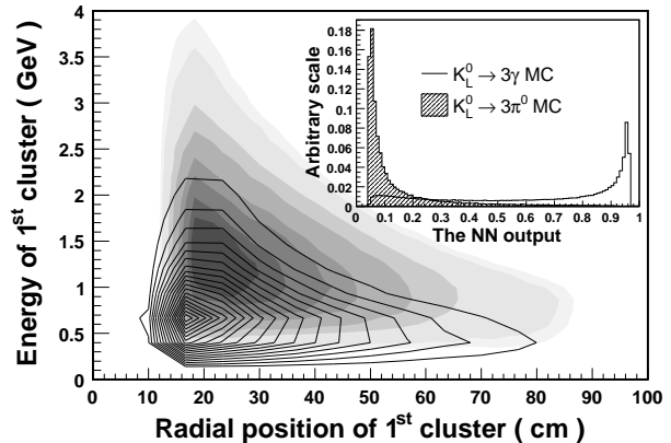
FIG. 4: Distribution of Cluster radial position vs. cluster energy of the MC events and the distributions of the NN output (sub-figure). The banded contour shows the K_L^0 \rightarrow 3\gamma parity-violating results, and the line contour shows the K_L^0 \rightarrow 3\pi^0 results. The significant differences in the distributions were also observed in the other two clusters.
