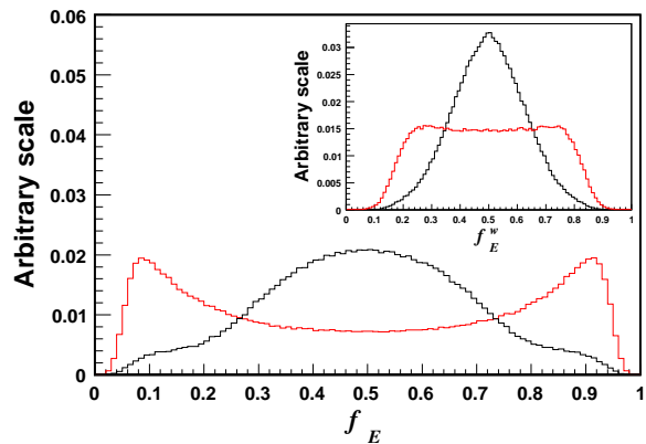
FIG. 2: Distributions of f_E and f_E^w (sub-figure) in the region of x' > 0 . The values of f_E and f_E^w were normalized by the total sum of f_E and f_E^w in all regions, respectively. The red histogram shows the distribution of single-photon clusters and the black histogram shows the distribution of fusion clusters. A significant difference between the distributions in the region of y' > 0 was also observed.
