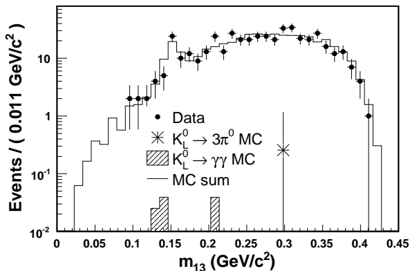
FIG. 5: Distributions of m_{13} of the events in the normalization region ( 0.13 \text{ GeV}/c^2 < m_{12} < 0.17 \text{ GeV}/c^2 ). The points with error bars show the data, the star sign shows the only survived K_L^0 \rightarrow 3\pi^0 MC event, and the shaded histograms show the K_L^0 \rightarrow \gamma\gamma MC events. The hollow solid histogram is the sum of the K_L^0 \rightarrow 3\pi^0 , K_L^0 \rightarrow \pi^0 \pi^0 and K_L^0 \rightarrow \gamma\gamma MC results.
