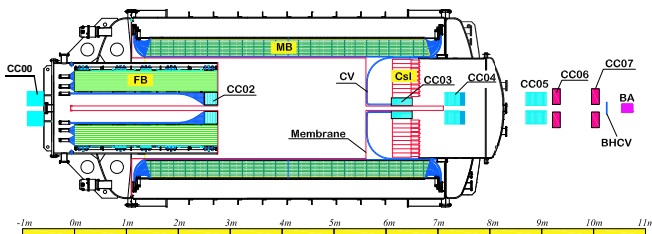
FIG. 1: Schematic cross-sectional view of the E391a detector. “0m” in the scale corresponds to the entrance of the front barrel (FB) detector. K_L^0 ’s entered from the left side.
