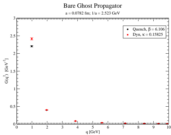
(c) Ghost propagator at a = 0.0782\text{fm} .
