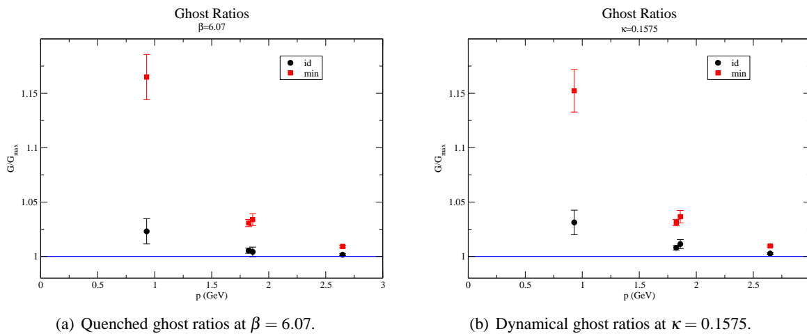
Figure 5: Ghost ratios.
