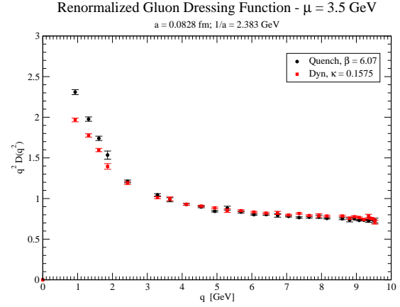
(b) Gluon dressing function at a = 0.0828 fm.
