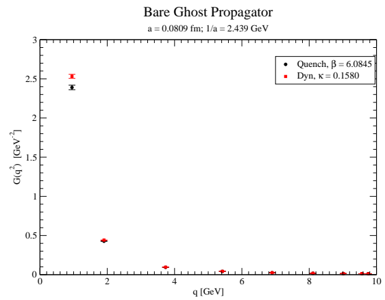
(b) Ghost propagator at a = 0.0809\text{fm} .
