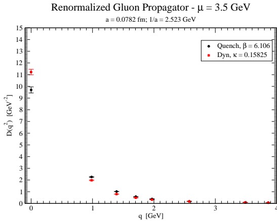
(e) Gluon propagator at a = 0.0782 fm.
