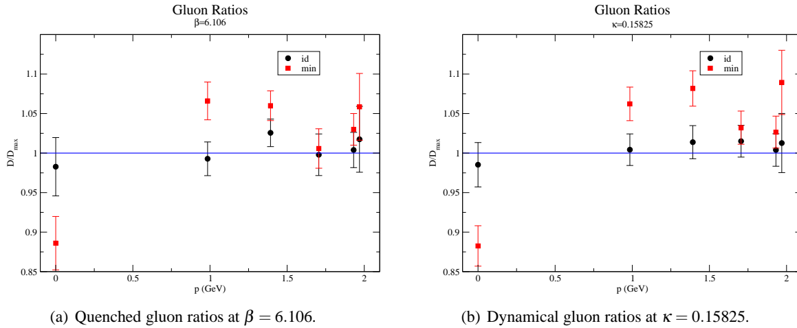
Figure 4: Gluon ratios.
