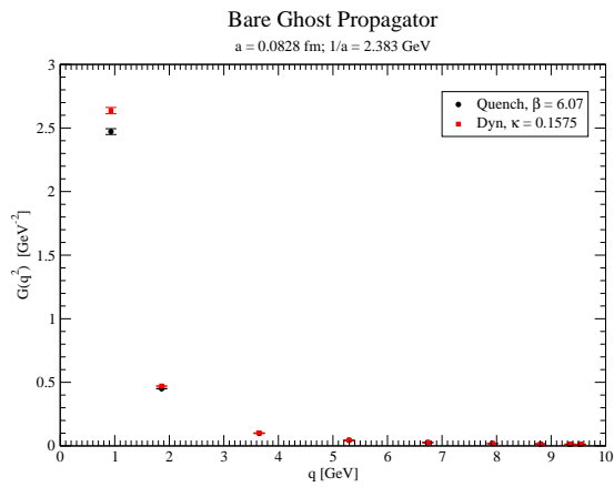
(a) Ghost propagator at a = 0.0828\text{fm} .
