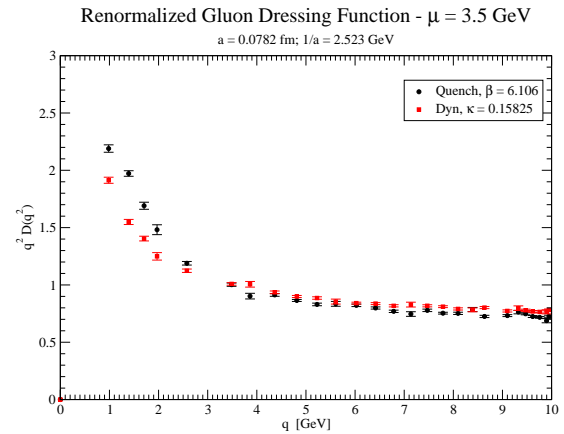
(f) Gluon dressing function at a = 0.0782 fm.
