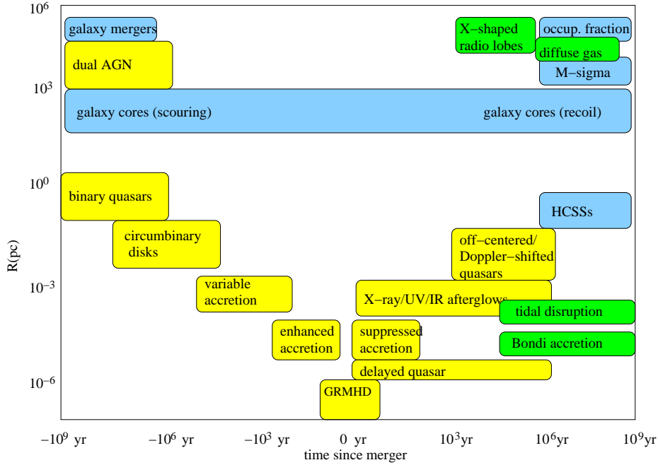
Figure 1. Selection of potential EM signatures, sorted by timescale, typical size of emission region, and physical mechanism (blue = stellar; yellow = accretion disk; green = diffuse gas/miscellaneous).
