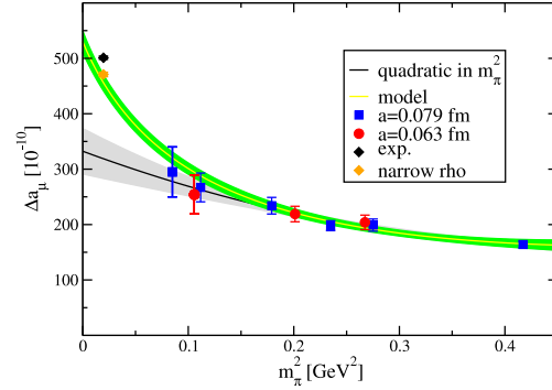
Figure 2: Vector contribution to \Delta a_\mu . A quadratic extrapolation in m_\pi^2 undershoots the measured contribution of the \rho significantly. A model (described in text) suggests the importance of calculating at small enough m_\pi for the vector mass to approach the physical \rho mass.
