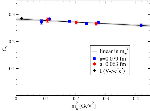
Figure 1: Vector coupling. The vector coupling, normalized as the \rho , calculated for a = 0.079 fm and a = 0.063 fm agree. A linear extrapolation in m_\pi^2 to the physical pion mass agrees with the value extracted from \Gamma(V \rightarrow e^+e^-) . The factor of m_V in f_V hides this agreement.
