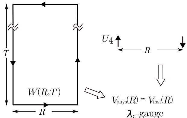
FIG. 4: The schematic illustration of the physical interquark potential V_{\text{phys}}(R) and the instantaneous potential V_{\text{inst}}(R) . In \lambda_C -gauge, the instantaneous potential V_{\lambda_C}(R) approximately reproduces the physical potential V_{\text{phys}}(R) .
