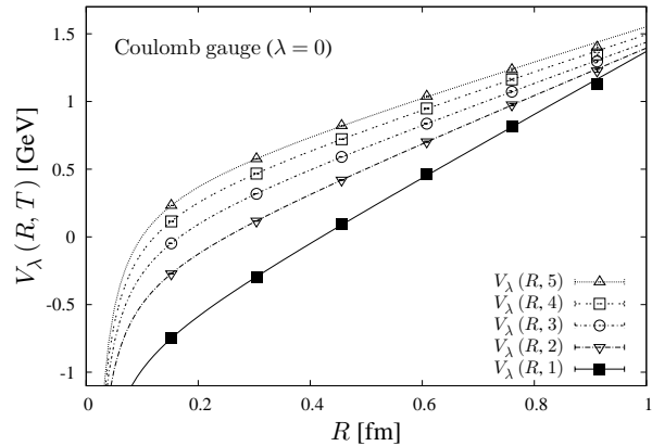
FIG. 5: “Finite-time potential” V_\lambda(R, T) in the Coulomb gauge ( \lambda = 0 ) for T=1,2,3,4,5 . Here, for the comparison, an irrelevant constant is shifted for each T . The curves denote the fit-results using the Coulomb plus linear form. The slope of V_\lambda(R, T) is clearly changed according to T .
