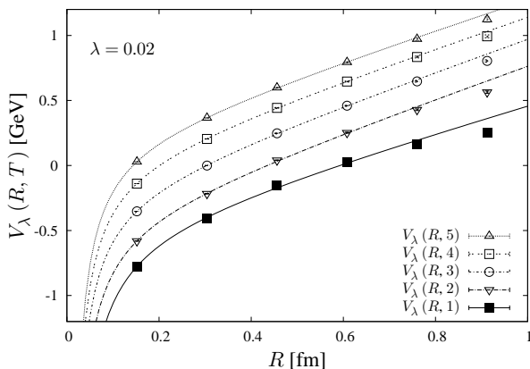
FIG. 7: Finite-time potential V_\lambda(R, T) at \lambda = 0.02 (\simeq \lambda_C) . For the comparison, an irrelevant constant is shifted for each T . The slope of V_\lambda(R, T) is almost the same for T = 1, 2, \dots, 5 , and thus the shape of V_\lambda(R, T) is rather stable against the temporal length T .
