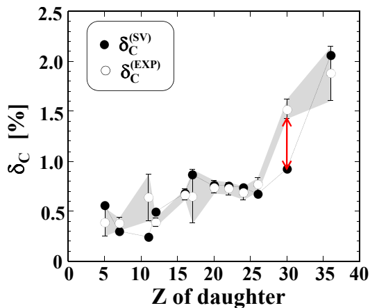
FIG. 2: (Color online) Calculated (black dots) and empirical (white dots, with error bars) values of \delta_C as function of proton number in the daughter nuclei. Vertical arrow marks the values for A = 62 . See text for details.
