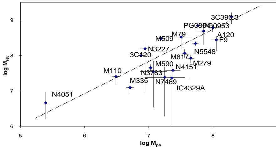
Fig. 2. Correlation between the BH mass measured by reverberation mapping, M_{rev} , and the mass M_{ph} estimated by the photo-ionization parameter combined with the Doppler widening of the H \beta line in a sample of Seyfert galaxies with reverberation data.
