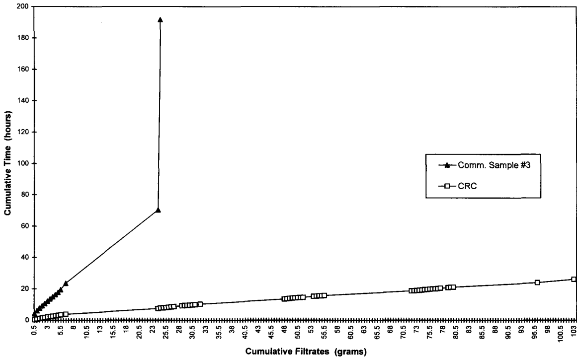
Figure 3. TLFP test (LSK method) prehydrated with tap water/ocean water as permeant.
