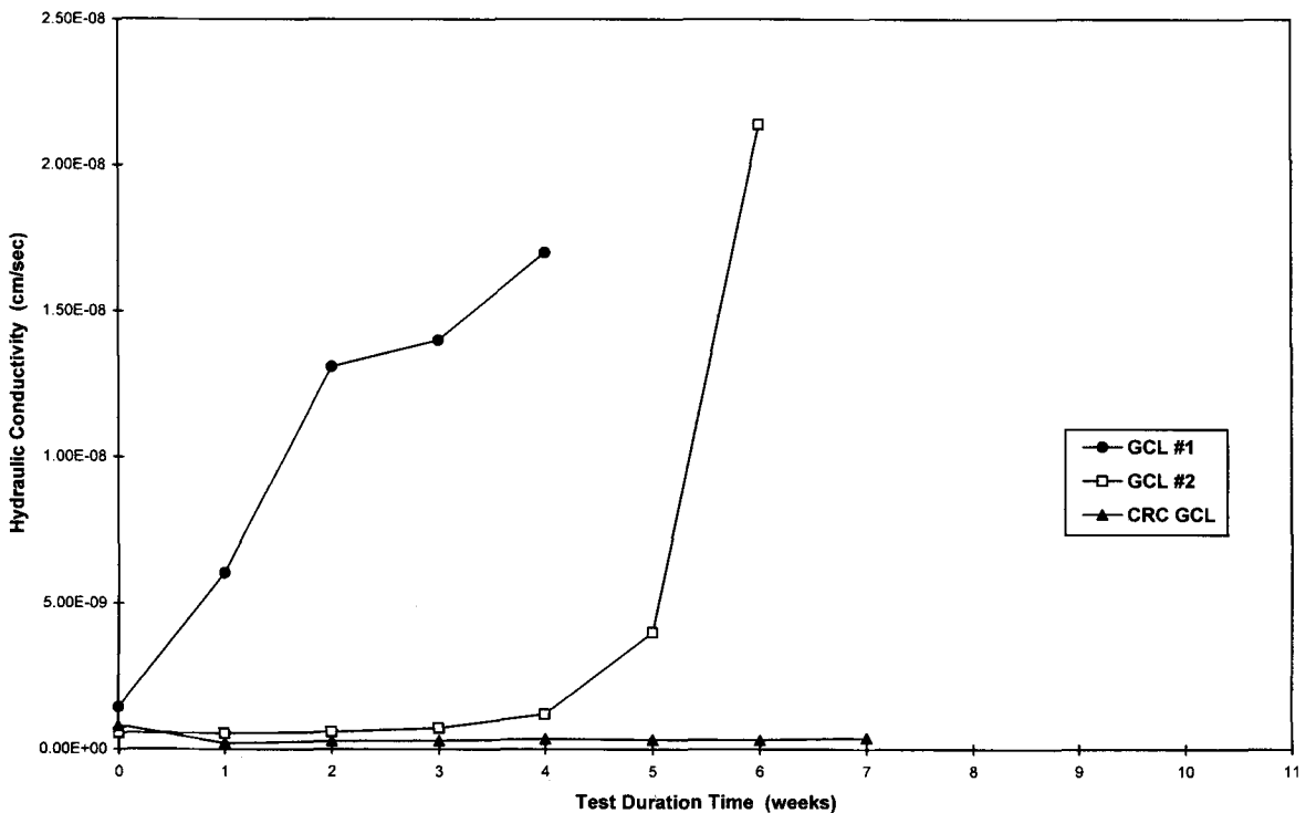
Figure 4. Flexible wall hydraulic conductivity test, prehydrated with 1000 ppm CaCl 2 /1% CaCl 2 as permeant.
