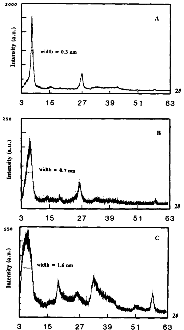
Figure 4. XRD patterns (CuKα) of A) saponite, B) hectorite, and C) laponite.
