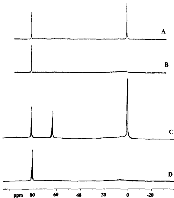
Figure 1. ^{27}\text{Al} -NMR spectra of Al-solutions: A) [\text{Al}^{3+}] = 0.1 \text{ M} ; R = 1 ; [\text{Ac}^-]/[\text{Al}^{3+}] = 0 ; B) [\text{Al}^{3+}] = 0.09 \text{ M} ; R = 1 ; [\text{Ac}^-]/[\text{Al}^{3+}] = 1 ; C) [\text{Al}^{3+}] = 0.5 \text{ M} ; R = 2 ; [\text{Ac}^-]/[\text{Al}^{3+}] = 0 ; and D) [\text{Al}^{3+}] = 0.5 \text{ M} ; R = 2 ; [\text{Ac}^-]/[\text{Al}^{3+}] = 5 .
