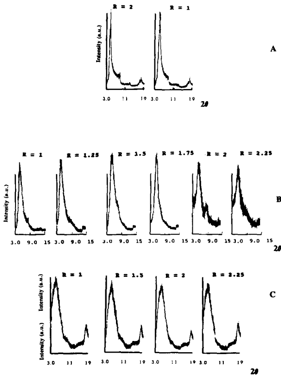
Figure 3. XRD patterns (CuKα) of clays pillared with refluxed solutions of different R-values: A) saponite; B) hectorite; and C) laponite.
