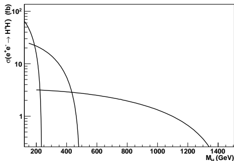
Figure 1: Higgs pair production: cross section for e^+e^- \rightarrow H^+H^- at \tan\beta = 20 as a function of M_{H^\pm} for \sqrt{s} = 0.5, 1.0 and 3.0 TeV.
