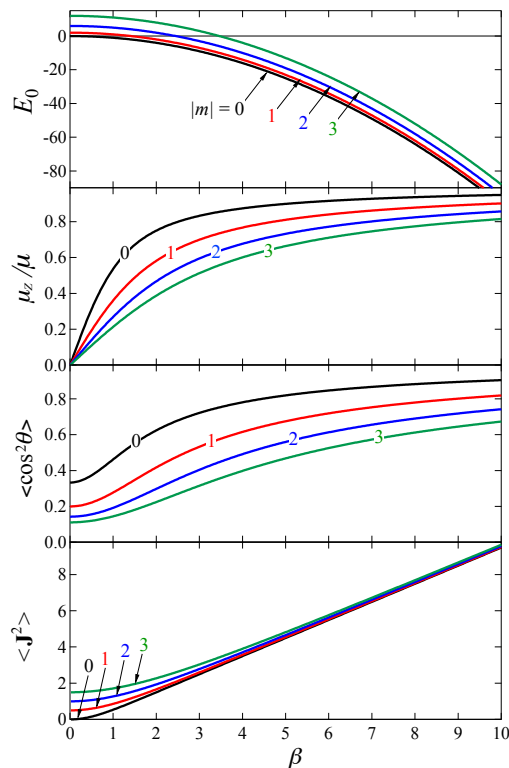
FIG. 3: Ground-state energies E_0 (in units of the rotational constant B ), space fixed dipole moments \mu_z/\mu \equiv \langle \cos \theta \rangle , alignment cosines \langle \cos^2 \theta \rangle , and expectation values of the angular momentum \langle \mathbf{J}^2 \rangle for different |\tilde{J} = m, m; \beta\rangle states as a function of the interaction parameter \beta .
