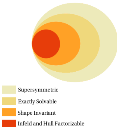
FIG. 4: A Venn diagram showing the relationships among supersymmetric, exactly solvable, shape invariant, and Infeld & Hull factorizable potentials.
