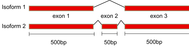
FIG. 7. A model gene for the study of Fisher information and accuracy of the single end and insert length models.
