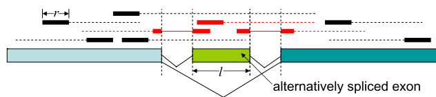
FIG. 2. Single end sequencing. A gene of three exons is shown with the middle exon of length l being alternatively spliced. Reads that come from this gene are shown above the gene in solid bars and the parts that are not sequenced are shown in broken lines. Reads that span an exon-exon junction are shown in solid bars connected by thin lines. Reads that are related to the AS exon are shown in red color. In this case only the reads in red are isoform informative.
