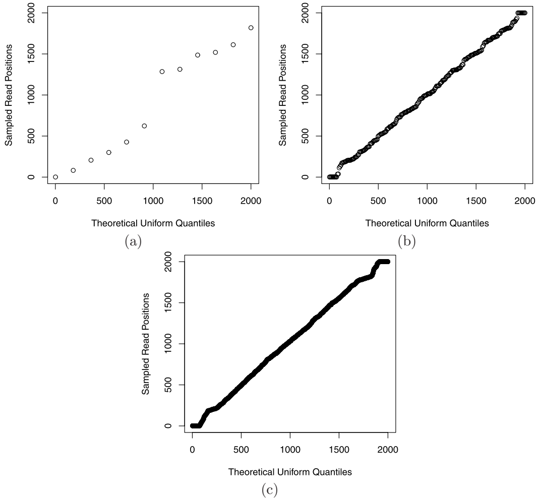
FIG. 4. Uniform Q - Q plot with sampled read positions. (a), (b) and (c) are generated by simulations with 10, 100 and 1,000 copies of transcripts, respectively.
