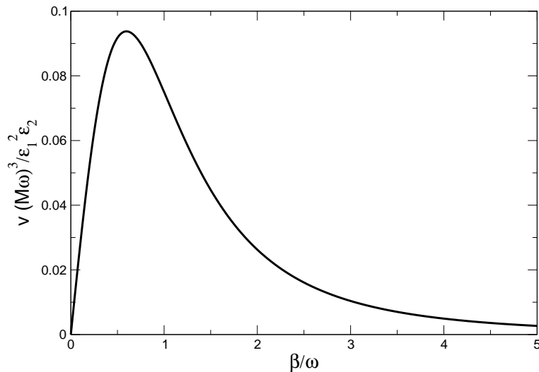
Figure 1. Plot of the current velocity v , in units of \epsilon_1^2\epsilon_2/(M\omega)^3 , vs. the damping coefficient \beta , in units of the frequency, \omega , induced by a biharmonic force like (1) with \phi_1 = \phi_2 = 0 . Notice that this force is time reversible, i.e., f(-t) = f(t) .
