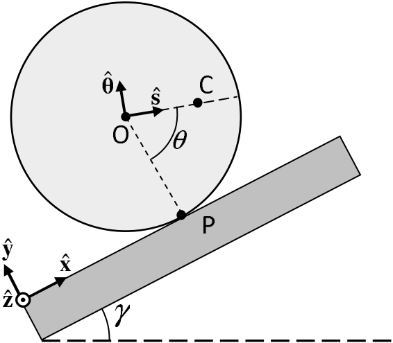
Figure 1. Rolling non-symmetric disk on a plane inclined at an angle \gamma to horizontal. O is the geometric center, C is the center of mass, P is the point of contact of the disk with the inclined plane, and \theta is the angle of the line through O and C with respect to perpendicular to the plane. Unit vector \hat{s} points from O to C , and \hat{\theta} = d\hat{s}/d\theta .
