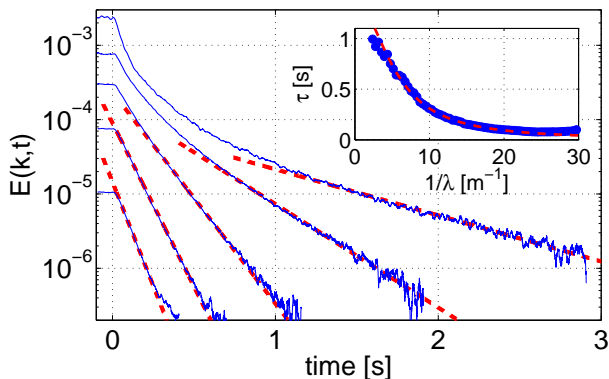
FIG. 3: Decay of energy. Main figure: evolution of the angle averaged power spectrum E(k, t) for 1/\lambda = k/2\pi = 5, 10, 15, 20, 25 \text{ m}^{-1} from top to bottom (semilog scale, the curves have been shifted vertically for clarity). Dashed lines: eye guides for the long time exponential decay of the energy. Insert: evolution of exponential decay times as a function of k . Dashed line: Lorentzian fit (0.73 + 0.025(k/2\pi)^2)^{-1} .
