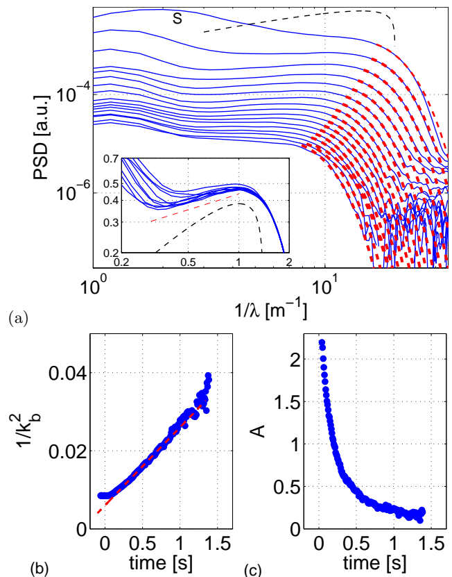
FIG. 2: (a) Decay of the velocity spectrum E(k = 2\pi/\lambda, t) at various times. Top solid curve (S): stationary spectrum. Lower solid curves, from top to bottom: 104 ms after stopping the forcing and every 83 ms subsequently (spectra are averaged over 42 ms). Thin dashed line at the top of the figure: shape of the theoretical spectrum ( E(k) \propto k \ln^{1/3}(k_c/k) ). Thick dashed line: fit of the model (3) for the dissipative part of the spectrum at each time. Insert : rescaling of the decaying spectra using the fitting parameter of (3) at each time as a function of k/k_b(t) (covering both the inertial and the dissipative range) for times between 0.1 and 0.83 s. Upper dashed line: power law k^{0.3} , lower dashed line: theoretical spectrum. (b) fitting parameter B/k_b^2(t) as a function of time. Dashed line: linear trend. (c) fitting parameter A as a function of time.
