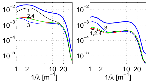
FIG. 4: Check of isotropy of the spectrum. (a) stationary forced regime. (b) decaying case after 0.18 s of decay. The upper thick curve is the fully angle averaged spectrum. The 4 lower curves correspond to an angle average over the 4 quadrants (see text). Curve 1 corresponds to propagation directions x^+ , curve 3 to x^- and 2 and 4 to both directions along y (almost superimposed).
