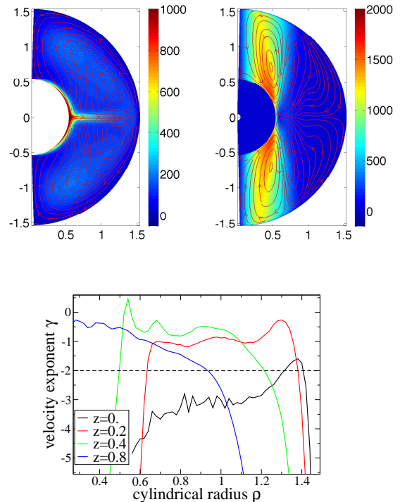
FIG. 7: Top: Structure of the spherical Couette flow when the outer sphere is now at rest, for \Lambda = 0 (left) and \Lambda = 2 (right), with Re = 5000 . Colors indicate azimuthal flow u_\phi and streamlines show the meridional recirculation. Note the absence of Stewartson layer in the purely hydrodynamical case (no global rotation) and the generation of the Shercliff layer in the magnetized one. Bottom: Velocity exponent \gamma taken at different altitude z , for \Lambda = 0 . Note the Rayleigh unstable profiles ( \gamma < -2 ) close to the midplane.
