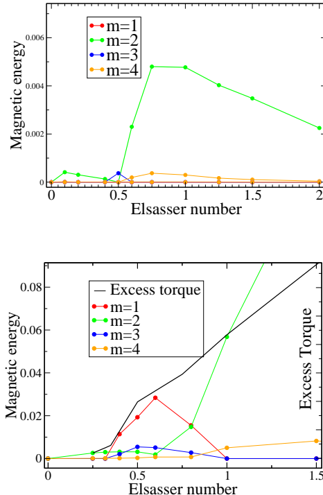
FIG. 9: Bifurcation diagram of the magnetic energy when \Lambda is increased, for Re = 5000 and Rm = 50 , with an outer sphere at rest and an axial applied magnetic field (Maryland experiment configuration). Top: insulating inner sphere. Bottom: conducting inner sphere. In the latter case, a good agreement with the Maryland experiment is obtained, including the generation of an m = 1 mode and increase of the torque on the inner sphere (to be compared with Fig.4 of [8]).
