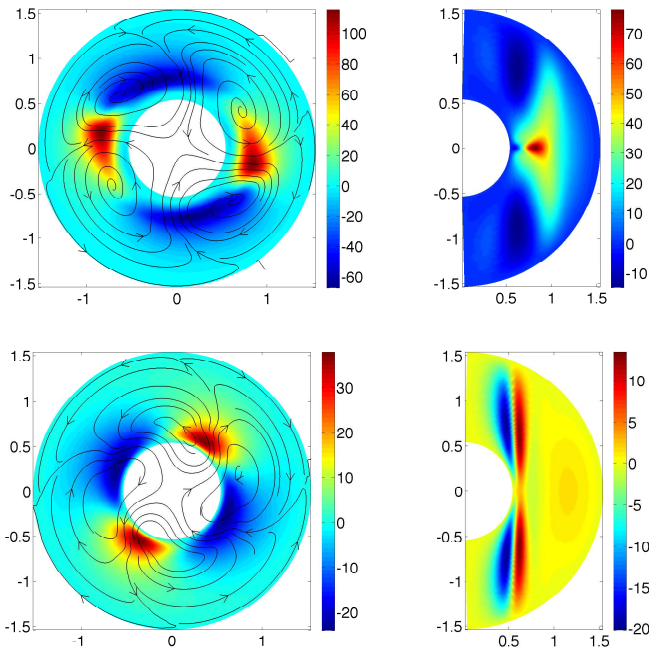
FIG. 10: Structure of the MHD instabilities for Re = 5000 with an insulating inner sphere and an axial field, formed of vortices in the horizontal plane. Figure shows the radial non-axisymmetric component of the velocity field u_r in the equatorial plane (left) or in a given meridional plane at \phi = 0 (right). The two top snapshots show the m = 2 mode obtained for \Lambda = 0.6 (instability related to the meridional return flow) and the two bottom snapshots show the field obtained for \Lambda = 2 . (Shercliff layer instability).
