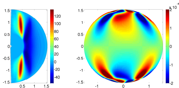
FIG. 12: Structure of the non-axisymmetric component of the Shercliff layer instability for Re = 5000 , Rm = 0.5 and \Lambda = 1.5 , with a conducting inner sphere. Left: non-axisymmetric u_r in the meridional plane \phi = 0 . Right: non-axisymmetric B_r at the surface of the outer sphere. Induction is not a necessary condition for the instability to be generated.
