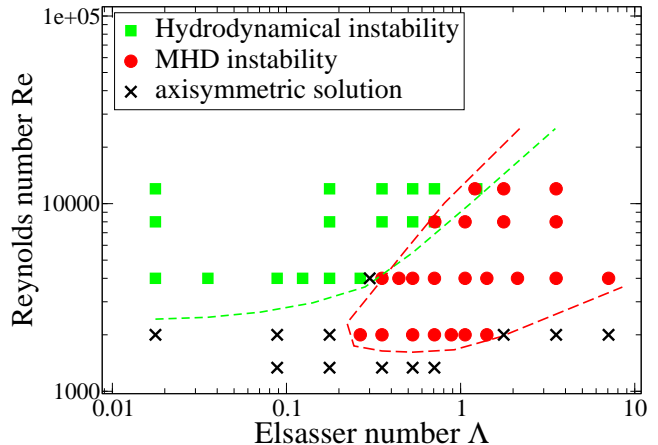
FIG. 2: Parameter space for a dipolar magnetic field applied to a system such that \Omega_i = 8\Omega_o , and with insulating spheres. Green squares indicate m = 2 hydrodynamical instabilities modified (and suppressed at large \Lambda ) by the applied field. Red circles are MHD instabilities of the return flow or the free shear layer triggered by the magnetic field, dominated by m = 1 and m = 2 azimuthal wavenumbers. Black crosses indicate classical spherical Couette solutions, purely axisymmetric.
