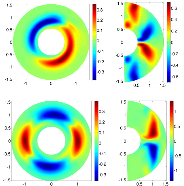
FIG. 5: Structure of the MHD instability for Re = 2000 . The figure shows the radial non-axisymmetric component of the magnetic field just above the equatorial plane (left) or in a given meridional plane at \phi = 0 (right). The two top figures show the m = 1 mode obtained for \Lambda = 0.35 and the two bottom figures show the field obtained for \Lambda = 0.9 , dominated by the m = 2 azimuthal wavenumber.
