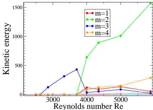
FIG. 8: Bifurcation diagram of the total kinetic energy when Re is increased. The outer sphere is at rest and Elsasser number is set to zero. As Re is increased, the equatorial jet adopts a wavy structure corresponding to non-axisymmetric modes, first m = 3 then m = 2 . For larger Re , it is expected that the flow tends to a fully turbulent state.
