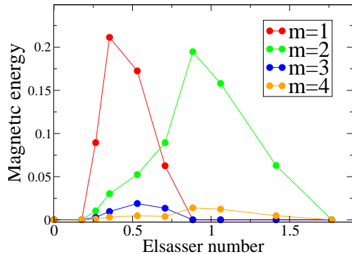
FIG. 4: Bifurcation diagram of the magnetic energy when the Elsasser number \Lambda is increased for a fixed Reynolds number Re = 2000 . Note the non-axisymmetric destabilization of the meridional return flow by the applied field, dominated by m = 1 and m = 2 non-axisymmetric modes. Strong applied fields suppress these MHD instabilities.
