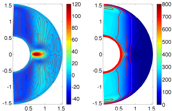
FIG. 1: Purely hydrodynamical Couette flow, obtained for Re = 2000 and \Omega_i/\Omega_o = 8 . Left: Radial component u_r of the axisymmetric velocity. Note the strong equatorial jet in the midplane. (lines represent streamlines of the axisymmetric poloidal recirculation). Right: angular velocity in the meridional plane, showing a broad Stewartson layer on the tangent cylinder. Contours of \Omega are also shown.
