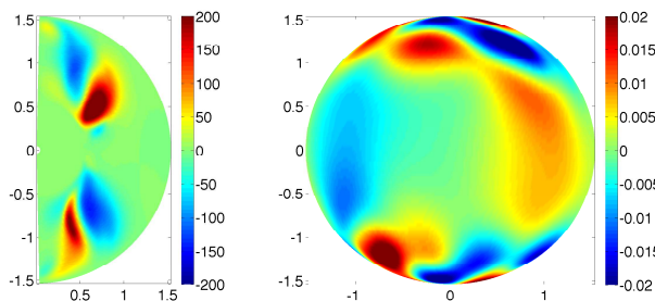
FIG. 11: Structure of the m = 1 instability obtained for \Lambda = 0.5 , Re = 5000 and Rm = 50 , in the case of a conducting inner sphere. Left: non-axisymmetric V_r in the meridional plane at \phi = 0 . Right: non-axisymmetric B_r at the surface of the outer sphere. The structure is identical to the mode observed in the Maryland experiment, with the same equatorial and azimuthal symmetries.
