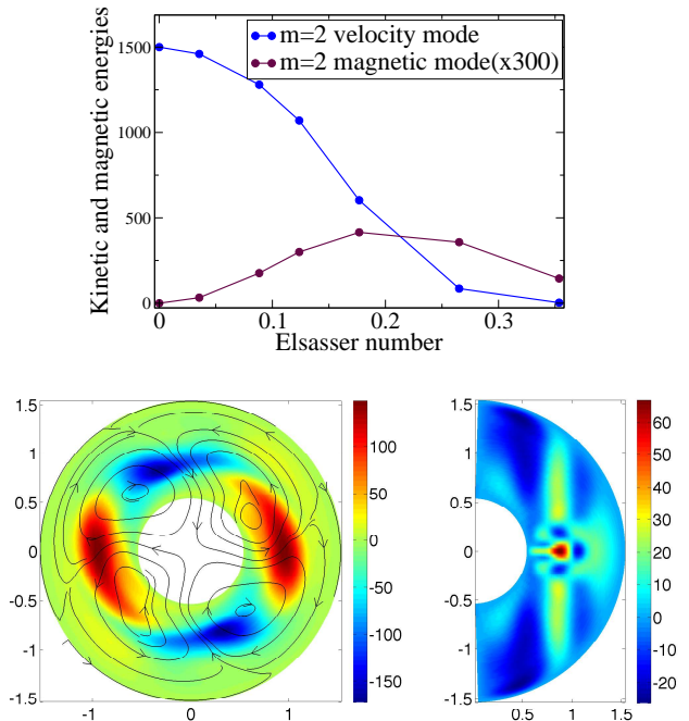
FIG. 3: Top: Evolution of magnetic and velocity modes when the Elsasser number is increased, for Re = 4000 .
