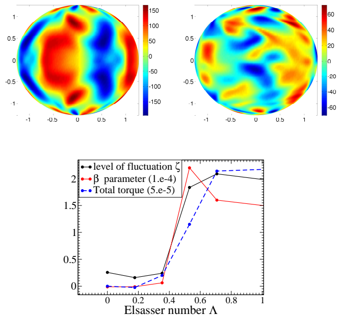
FIG. 6: Effect of the imposed magnetic field on the turbulence level, for Re = 8000 and \Omega_i = 8\Omega_o . Top: non-axisymmetric u_\phi at the spherical surface of radius r = 1.2 showing that for \Lambda = 0 (left), the flow is dominated by an m = 2 mode due to a hydrodynamic instability, and is weakly fluctuating. Right: For \Lambda = 1 , when boundary-driven instabilities are generated by the applied field, the flow becomes more complicated and chaotic. Bottom: evolution of the turbulence intensity when the magnetic field is increased. MHD instabilities due to boundaries yield turbulent fluctuations and angular momentum transport, similarly to the MRI.
