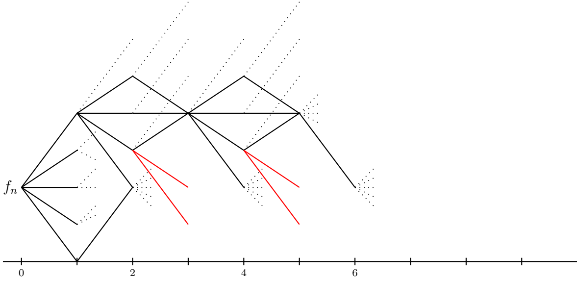
FIGURE 3. ( q = 4 ) According to Lemma 3.5, the sum of (the iterated contractions represented by) those walks which run on a red line tends to 0.
