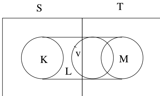
Figure 1: The rolling ball method
