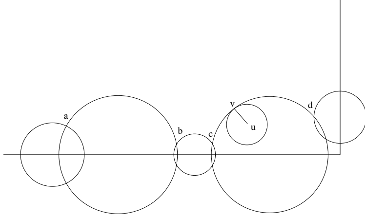
Figure 3: Some discs used in the construction of R
