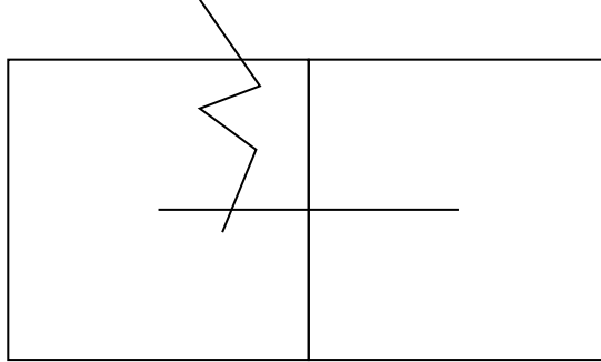
Figure 2: Forbidden path for upper bound method
