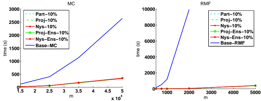
Figure 2: Speed-up of SUBMF relative to base algorithms.
