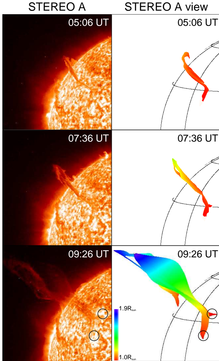
Fig. 3.— Comparison of the observed filament (left panels) and the reconstructed filament (right panels) seen from the STEREO A view. The black circles denote the western endpoints of the filament.
