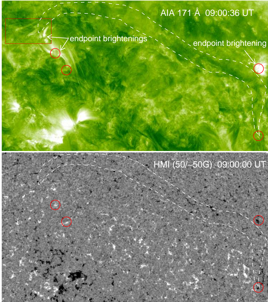
Fig. 9.— AIA 171 Å image (upper panel) and HMI line-of-sight magnetogram (lower panel) at the filament location. The white contours are the filament at 05:06 UT. The red circles denote the multiple endpoints of the filament. The red rectangle is the 171 Å image at 07:40 UT.
