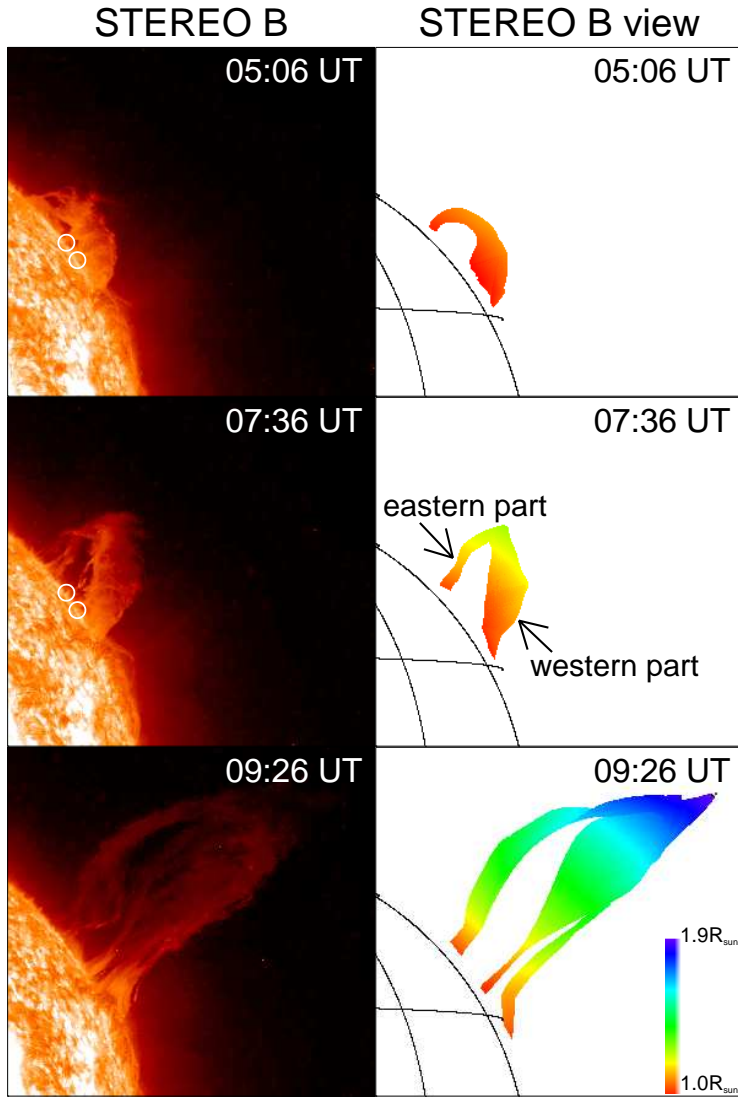
Fig. 4.— Comparison of the observed filament (left panels) and the reconstructed filament (right panels) seen from the STEREO B view. The white circles denote the barbs of the filament.
