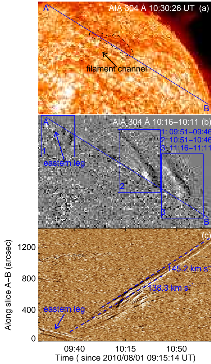
Fig. 10.— Appearance of the second eruption of filament material seen in AIA 304 Å (panel (a)) and running-difference images (panel (b)) and the running ratio stack plot obtained along slice A-B (panel (c)). The black contour denotes the filament material along line A-B.
