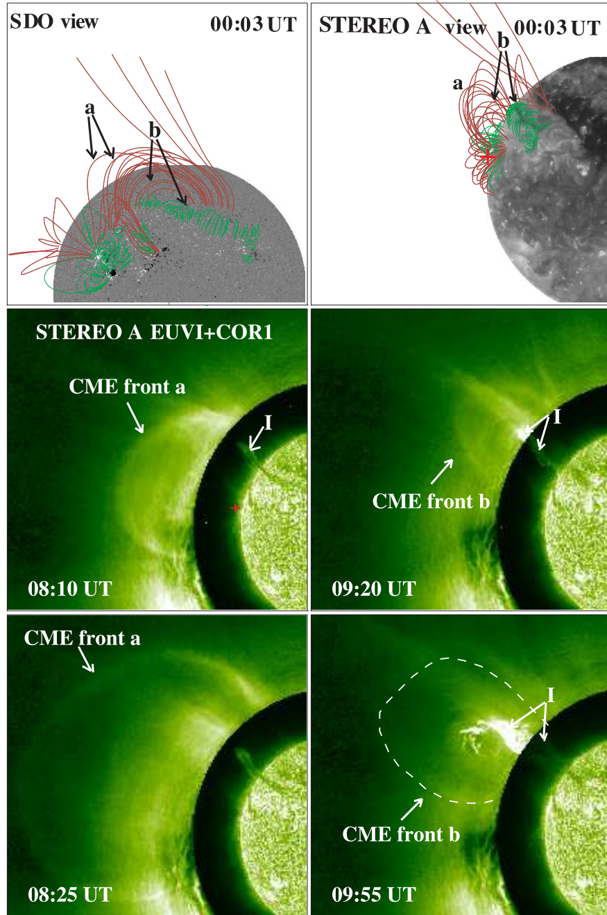
Fig. 1.— Extrapolated coronal magnetic field lines seen from the SDO (top left) and STEREO A (top right) perspectives at 00:03 UT on 2010 August 1 and composite images (middle and bottom panels) of STEREO-A COR1 and EUVI 304 Å. The backgrounds in the top panels are the MDI line-of-sight magnetogram at 00:03 UT and the STEREO A 195 Å image at 00:05 UT, respectively. Characters “a” and “b” denote the large-scale and small magnetic structures. Red and green curves represent high and low magnetic lines. Arrows “I” indicate the filament material. The plus signs denote the flare position.
