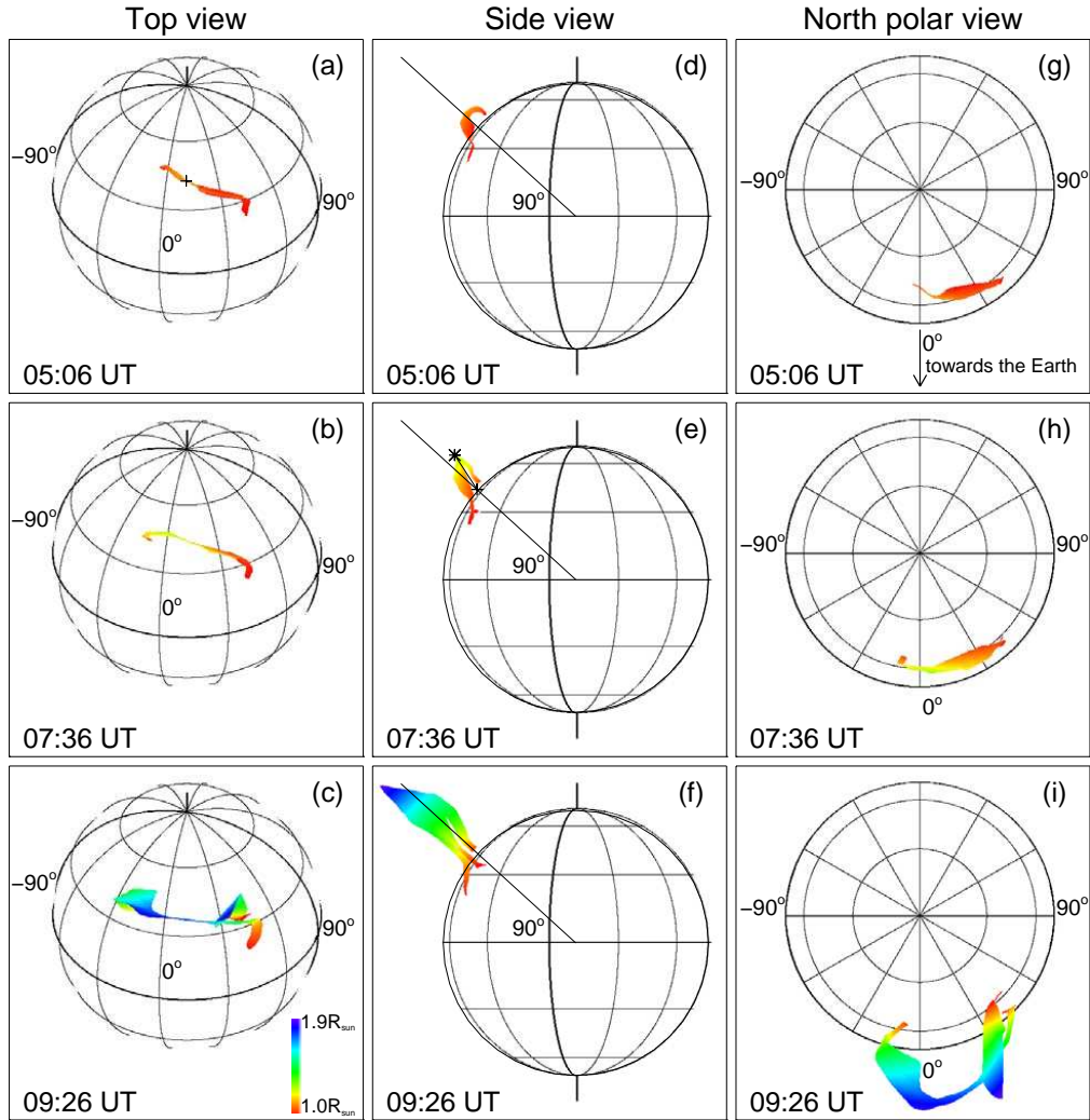
Fig. 5.— Evolution of the reconstructed filament seen from the top view (left panels), the side view (middle panels) and the north polar view (right panels). In the heliographic coordinate system, the top view of the filament has a longitude of 12^\circ and a latitude of 39^\circ , and the side view has a longitude of 102^\circ and a latitude of 0^\circ .
