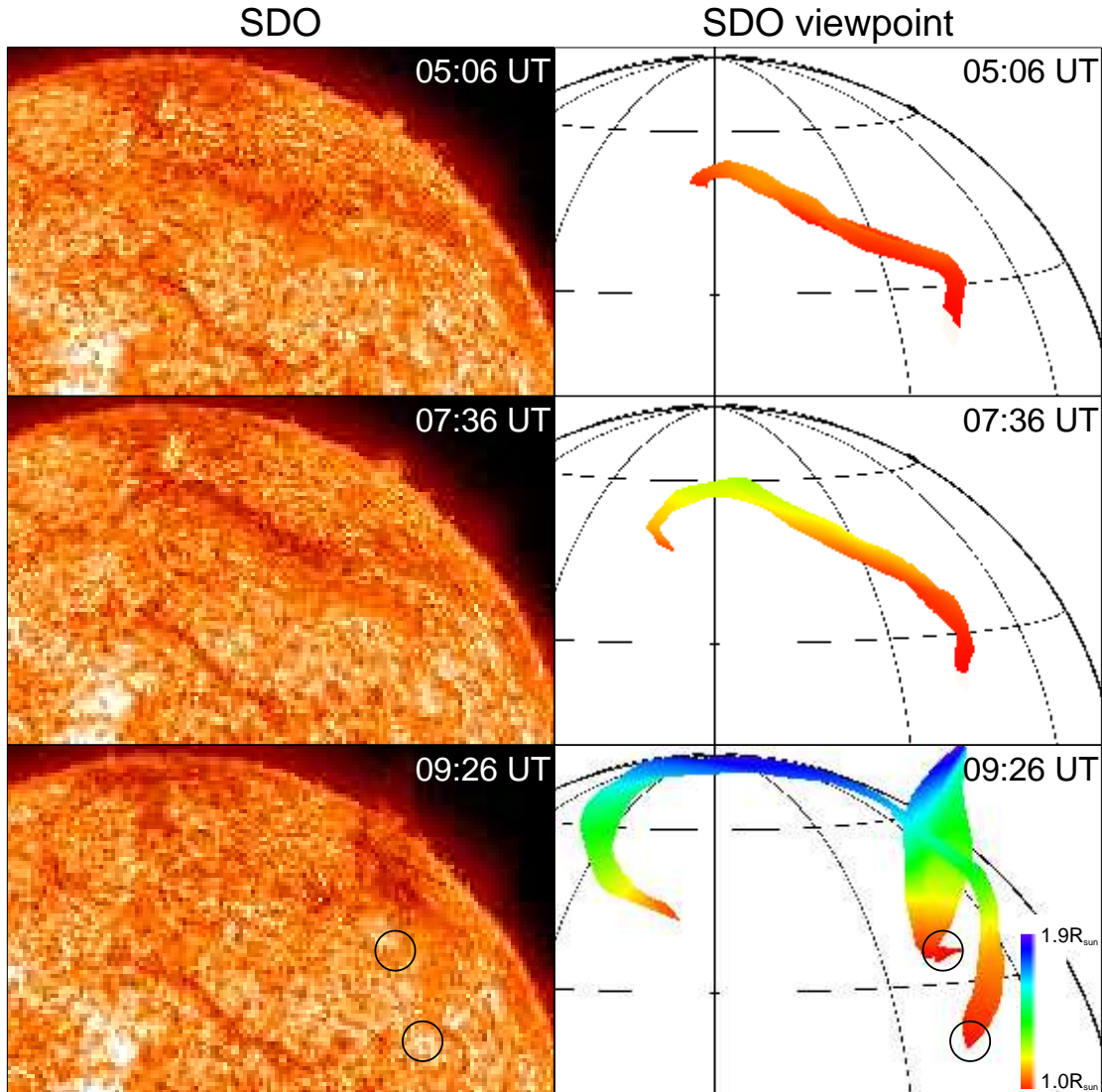
Fig. 2.— Reconstructed filament seen from the SDO viewpoint. Left: a series of SDO/AIA 304 Å observed images showing the evolution of the filament. Right: a series of reconstructed images seen from the SDO viewpoint showing the eruption process of the filament. The black circles denote the western endpoints of the filament.
