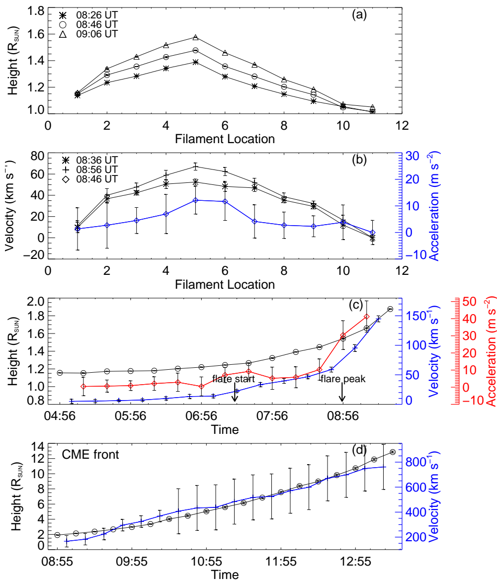
Fig. 7.— (a): True height-location plots of the 11 points (points “1” to “11” in Figure 6) at three different times. (b): Velocity-location and acceleration-location plots of the 11 points. (c): True height-time, velocity-time and acceleration-time plots of the highest point between 04:56 UT and 09:36 UT. (d): Projected height-time and velocity-time plots of the associated CME measured in STEREO A/COR1 and COR2 images.
