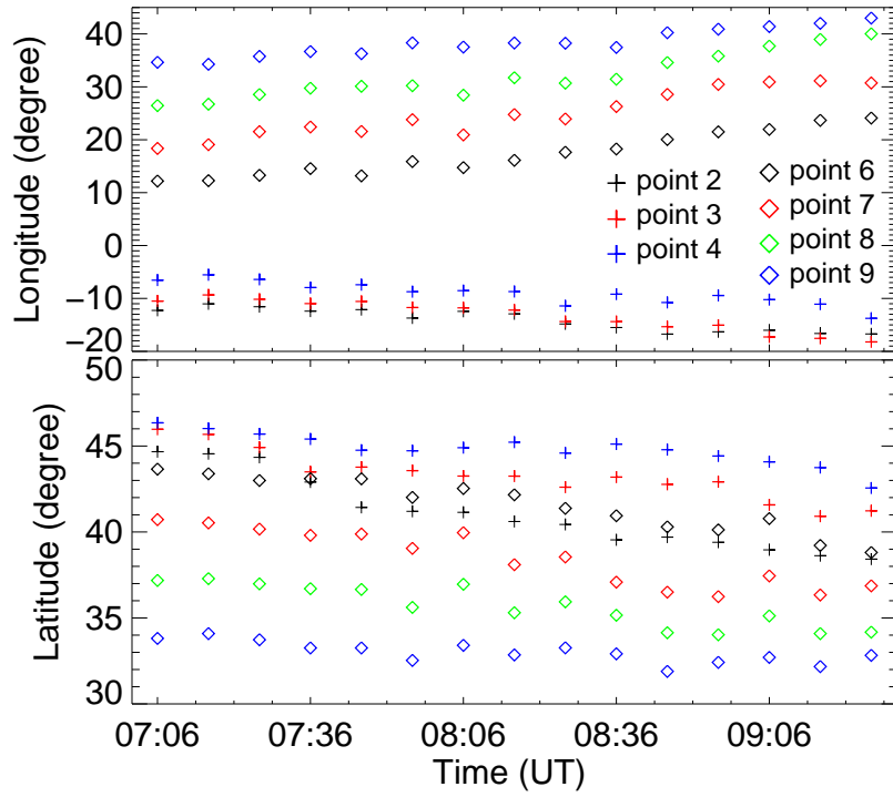
Fig. 8.— Longitude-time and latitude-time plots of different points of the filament. Points “2” to “4” are from the eastern leg, and points “6” to “9” are from the western leg (Figure 6).
