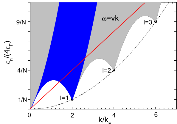
FIG. 1. (Color online) Schematic of the excitation spectrum of the 1D Bose gas in a perfectly isotropic ring. The supercurrent states I lie on the parabola \hbar^2 k^2 / (2Nm) (dotted line). Excitations occur in the shaded area; the discrete structure of the spectrum is not shown for simplicity. The blue (dark) area represents single particle-hole excitations [28]. Motion of the impurity with respect to the gas causes transitions from the ground state to the states lying on the straight (red) line. Reproduced from Ref. [31], Copyright ©2009 The American Physical Society
