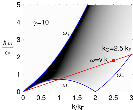
FIG. 4. (Color online) Numerical values of the DSF (4) for the coupling parameter \gamma = 10 [59]. The dimensionless value of the rescaled DSF S(k, \omega)\epsilon_F/N is shown in shades of gray between zero (white) and 1.0 (black). The upper and lower solid (blue) lines represent the dispersions \omega_+(k) and \omega_-(k) , respectively, limiting the single “particle-hole” excitations in the Lieb-Liniger model at T = 0 . The dispersions are obtained numerically by solving the system of integral equations [28]. The gray scale plot of the DSF demonstrates that the main contribution to the DSF comes from the single particle-hole excitations, lying inside the region \omega_-(k) \leq \omega \leq \omega_+(k) (see also Fig. 1). Only one point at k = k_G , shown in full (red) circle, contributes to the integral when the perturber is a shallow cosine potential with a reciprocal vector k_G . Reproduced from Ref. [31], Copyright ©2009 The American Physical Society
