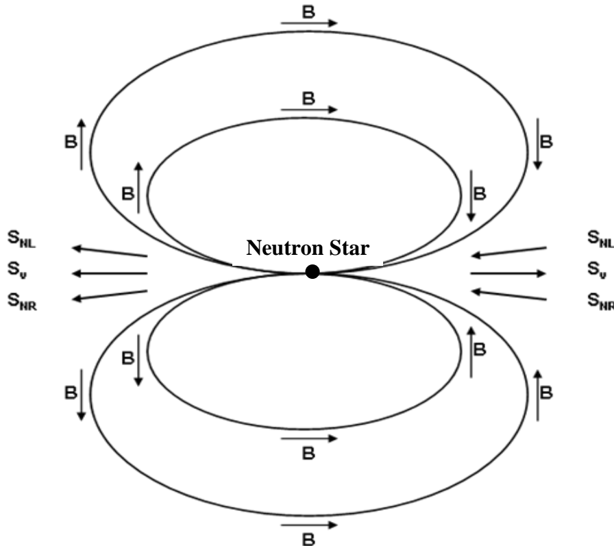
Figure 1. Schematic diagram of the magnetic fields, \underline{B} , surrounding a nascent neutron star and the spins of the {}^{14}\text{N} nuclei, S_N , and of the neutrinos, S_\nu , emitted from the supernova that created the neutron star.
