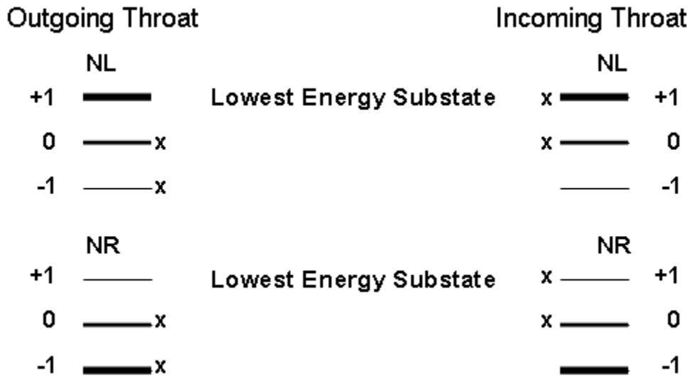
Figure 2. Magnetic substate distributions for ^{14}\text{N} nuclei resulting from the Buckingham effect. The “x” indicate the states that will undergo greater processing from the electron antineutrinos. NL refers to left-handed ^{14}\text{N} nuclei, and NR to the right-handed ^{14}\text{N} nuclei. “Outgoing (Incoming) throat” refers to the throat of the neutron star at which the magnetic field is outgoing (incoming). The thickness of the line for each substate indicates its relative population.
