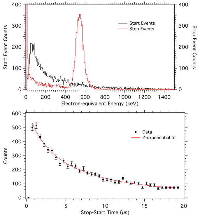
Figure 4: Results from a demonstration of the {}^6\text{Li} -loaded liquid scintillator cell irradiated by a {}^{252}\text{Cf} source. The top plot shows the energy distribution of the start events (primarily recoil events) and stop events (primarily capture on {}^6\text{Li} ). The peak in the spectrum of stop events corresponds to the total energy of the {}^6\text{Li} reaction products. The bottom plot shows the delay time (between start and stop events) distribution for event sequences where the stop event produces light consistent with neutron capture on {}^6\text{Li} . The error bars represent plus and minus the combined standard uncertainty.
