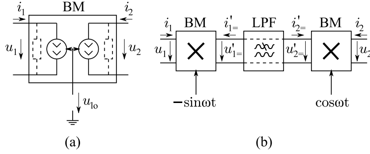
FIG. 2: (a) Equivalent circuit of an idealized balanced modulator (BM). (b) A network composed of two balanced modulators connected through a low-pass filter (LPF).
