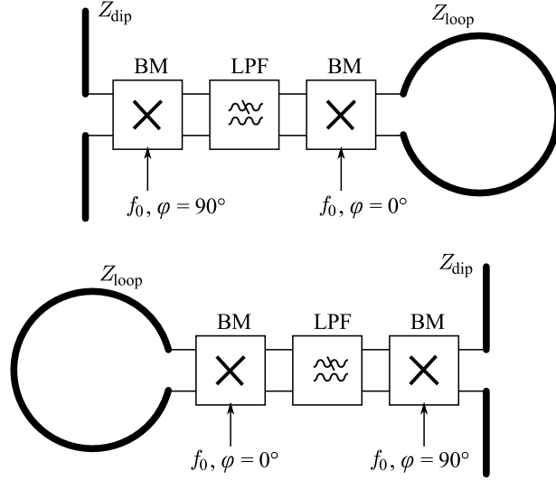
FIG. 3: The topology of the two types of phase conjugating bi-anisotropic inclusions for the phase conjugating surface operating at the frequency f_0 . Each particle consists of a short dipole antenna with the impedance Z_{\text{dip}} and a small loop antenna with the impedance Z_{\text{loop}} . The two antennas are interconnected through a nonlinear and nonreciprocal network composed of two balanced modulators (BM) and a low-pass filter (LPF). The mixers are fed by a local oscillator with two signal outputs in quadrature \varphi = 0^\circ and \varphi = 90^\circ . See the main text for further explanations.
