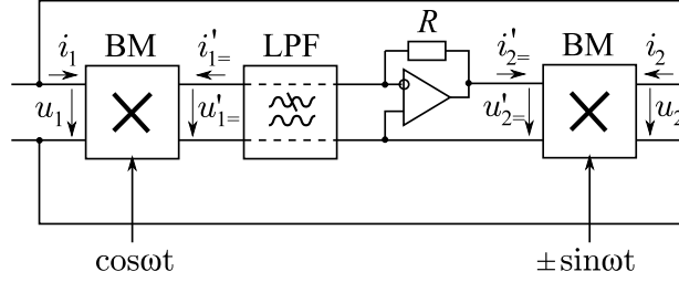
FIG. 4: A nonlinear single-port network used as a load for a short electric dipole. The network is composed of the same elements as in Fig. 2, with an additional operational amplifier working in the current-to-voltage conversion mode.
