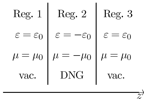
FIG. 1: An ideal Veselago lens: A planar slab of a double-negative (DNG) material with the medium parameters \varepsilon = -\varepsilon_0 and \mu = -\mu_0 in free space.
