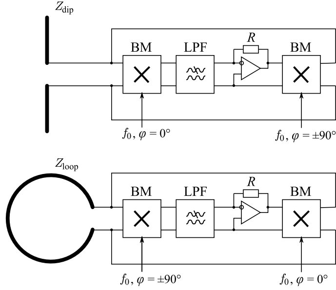
FIG. 5: The topology of the two particles loaded with nonlinear circuits designed to operate with the evanescent part of the spatial spectrum. Top: a short electric dipole loaded with a nonlinear load. Bottom: a small magnetic loop loaded with a nonlinear load.
