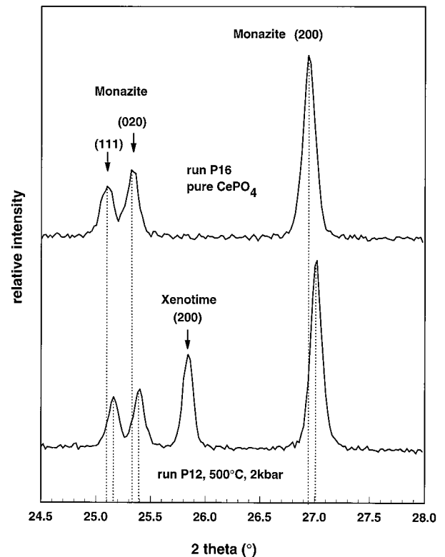
FIGURE 7. Portion of the X-ray patterns of experiment P16 (pure \text{CePO}_4 end-member) and P12 (coexisting monazite and xenotime). The (111), (020), and (200) reflections of monazite show identical half width. Peaks of P12 are shifted to higher 2\theta values because of incorporation of 5 \pm 1 mol% Y into the monazite structure. The pattern of P12 shows also the (200) reflection of xenotime.
