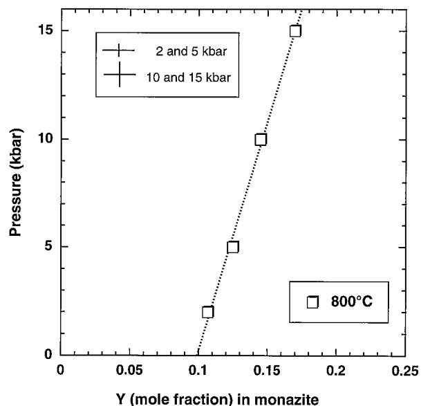
FIGURE 9. X_{\text{Y}}^{\text{monazite}} -pressure plot depicting the pressure dependence of the monazite limb of the miscibility gap at 800 °C. Data points are from reaction products that contained monazite plus xenotime. Values are from Table 1.
