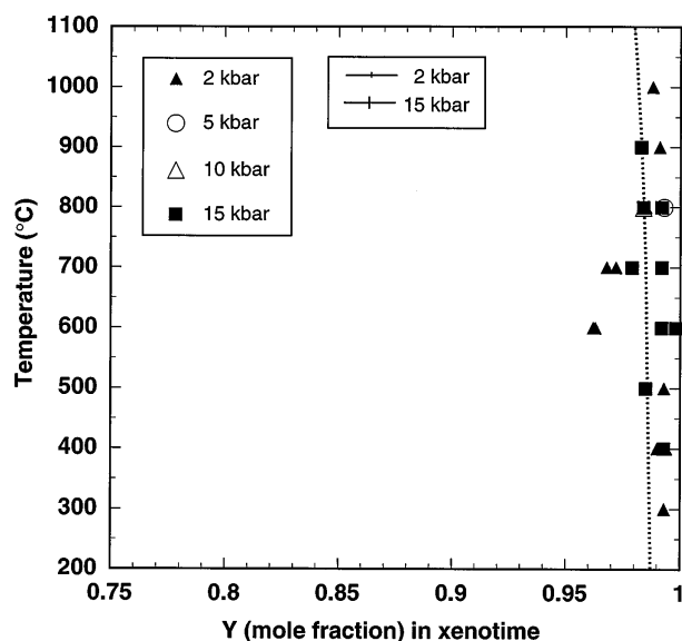
FIGURE 10. X_{\text{Y}}^{\text{xenotime}} -temperature plot depicting the xenotime limb of the monazite-xenotime miscibility gap at 2 kbar (black triangles) and 15 kbar (black squares). All data points are from reaction products that contained monazite plus xenotime. Values are from Table 1.
