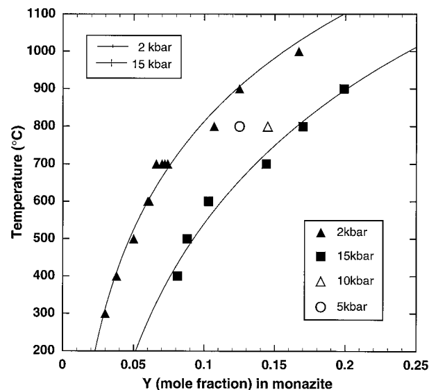
FIGURE 8. X_{\text{Y}}^{\text{monazite}} -temperature plot depicting the monazite limb of the monazite-xenotime miscibility gap at 2 kbar (black triangles) and 15 kbar (black squares). All data points are from reaction products that contained monazite plus xenotime. Values are from Table 1.
