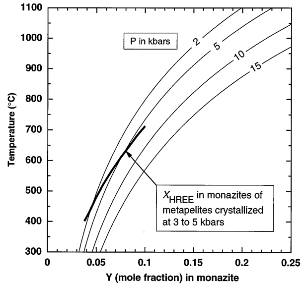
FIGURE 12. X_{\text{Y}}^{\text{monazite}} -temperature plot showing the monazite limb of the miscibility gap at various pressures, calculated using Equation 1. Thick curve indicates the mole fraction of Y + HREE (Gd-Lu) of natural monazites from a metapelite suite that crystallized together with xenotime at about 400–700 °C and about 3 to 5 kbar (Heinrich et al. 1997). The monazite limb of the (Ce-Y) \text{PO}_4 binary and that of the (LREE-HREE,Y) \text{PO}_4 system in rocks almost coincide within error limits (see Fig. 7).
