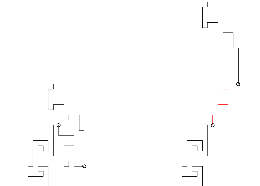
FIGURE 4. In the left-hand sketch, an element of SAB_n and one of its zigzags is illustrated. The zigzag's central section is shown in red and the points of zig and of zag are marked by dots. The unfolding of the walk indexed by this zigzag is depicted on the right.
