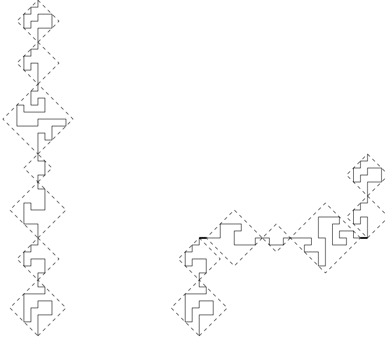
FIGURE 3. The stickbreak operation is depicted. Note the two east-west edges, depicted in bold, that are inserted at either end of the rotated section in order to ensure that the outcome of the operation is self-avoiding.
