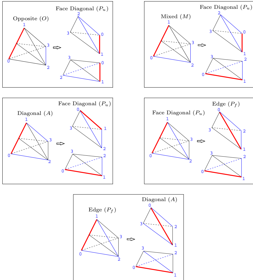
Figure 2: Refinement rules for the 5 refinement types
