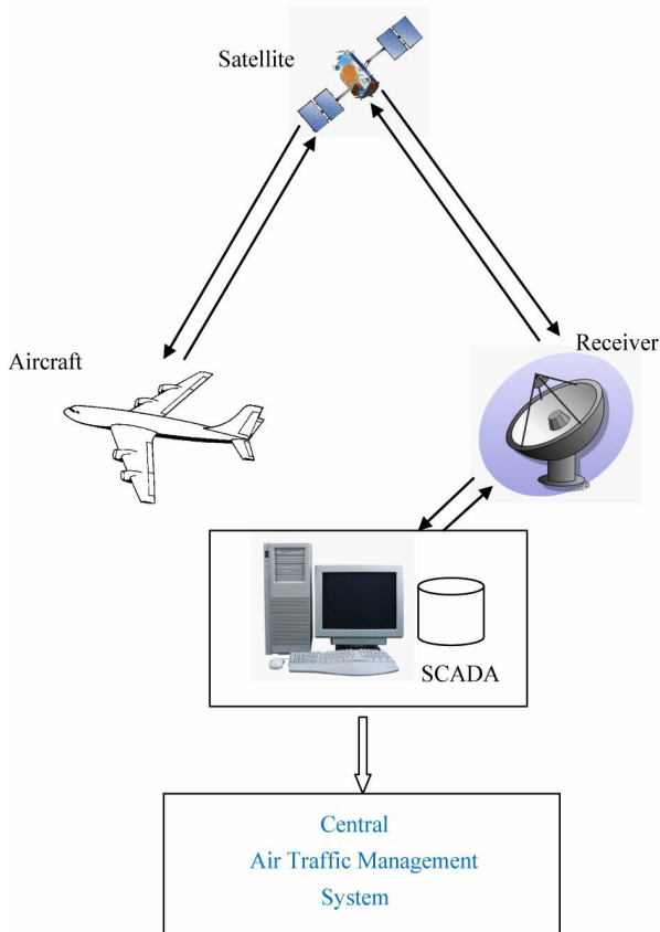
Figure 1. A schematic diagram of the digital information system.
