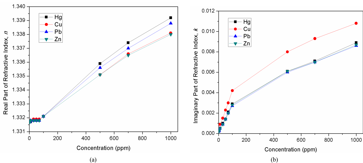
Figure 8. (a) The real part of refractive index, n , as a function of \text{Hg}^{2+} , \text{Cu}^{2+} , \text{Pb}^{2+} and \text{Zn}^{2+} concentration. (b) The imaginary part of refractive index, k , as a function of \text{Hg}^{2+} , \text{Cu}^{2+} , \text{Pb}^{2+} and \text{Zn}^{2+} concentration.
