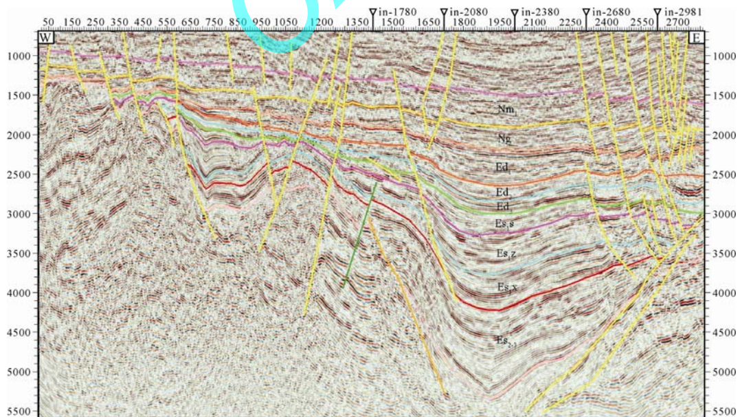
图 2 北大港构造带东翼港东—白东地震剖面(Crossline 480 测线, 位置见图 1) (W: (x: 20535000, y: 4280000), E: (x: 20580000, y: 4305000)) Fig. 2 Seismic section of Gangdong-Baidong in eastern Beidagang tectonic belt(For position of the measuring line 480 see Fig. 1) (W: (x: 20535000, y: 4280000), E: (x: 20580000, y: 4305000))
