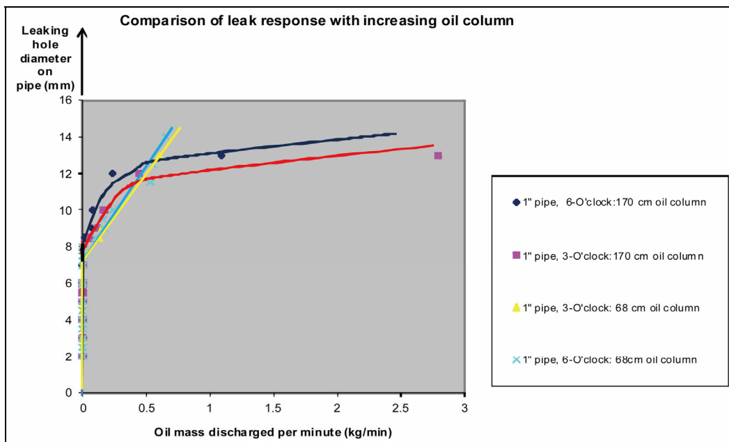
Figure 4. Comparing leak characteristics for varying oil column.
