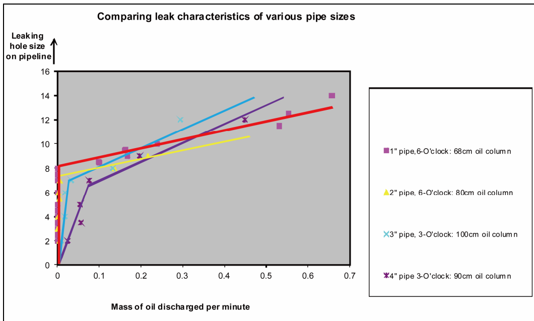
Figure 3. Plot of leak characteristics of various pipe size.
