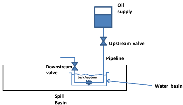
Figure 1. Test of leakage in water.
