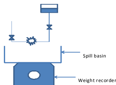
Figure 2. General test set-up (onshore).
