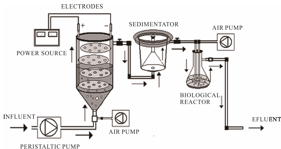
Figure 1. Electrocoagulations- Chytriomycetes hyalinus continuous system.
