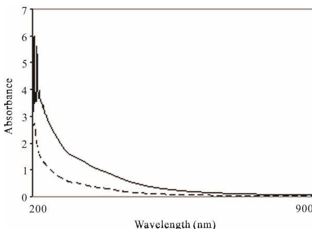
Figure 5. UV visible characterizations of industrial wastewater before (—) and after (----) electrocoagulations- Chytriomycetes hyalinus treatment.
