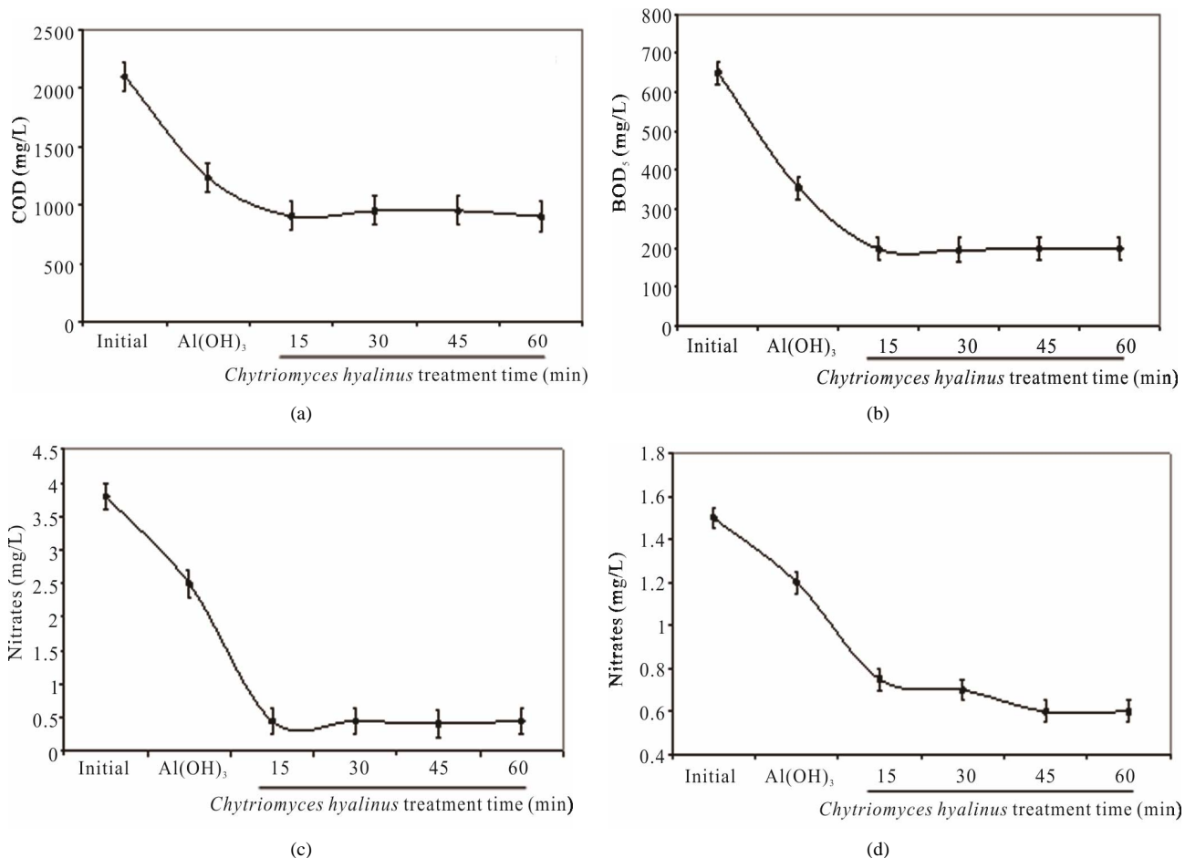
Figure 3. (a) COD, (b) BOD 5 , (c) nitrates and (d) nitrites during the electrochemical- Chytriomycetes hyalinus treatment.
