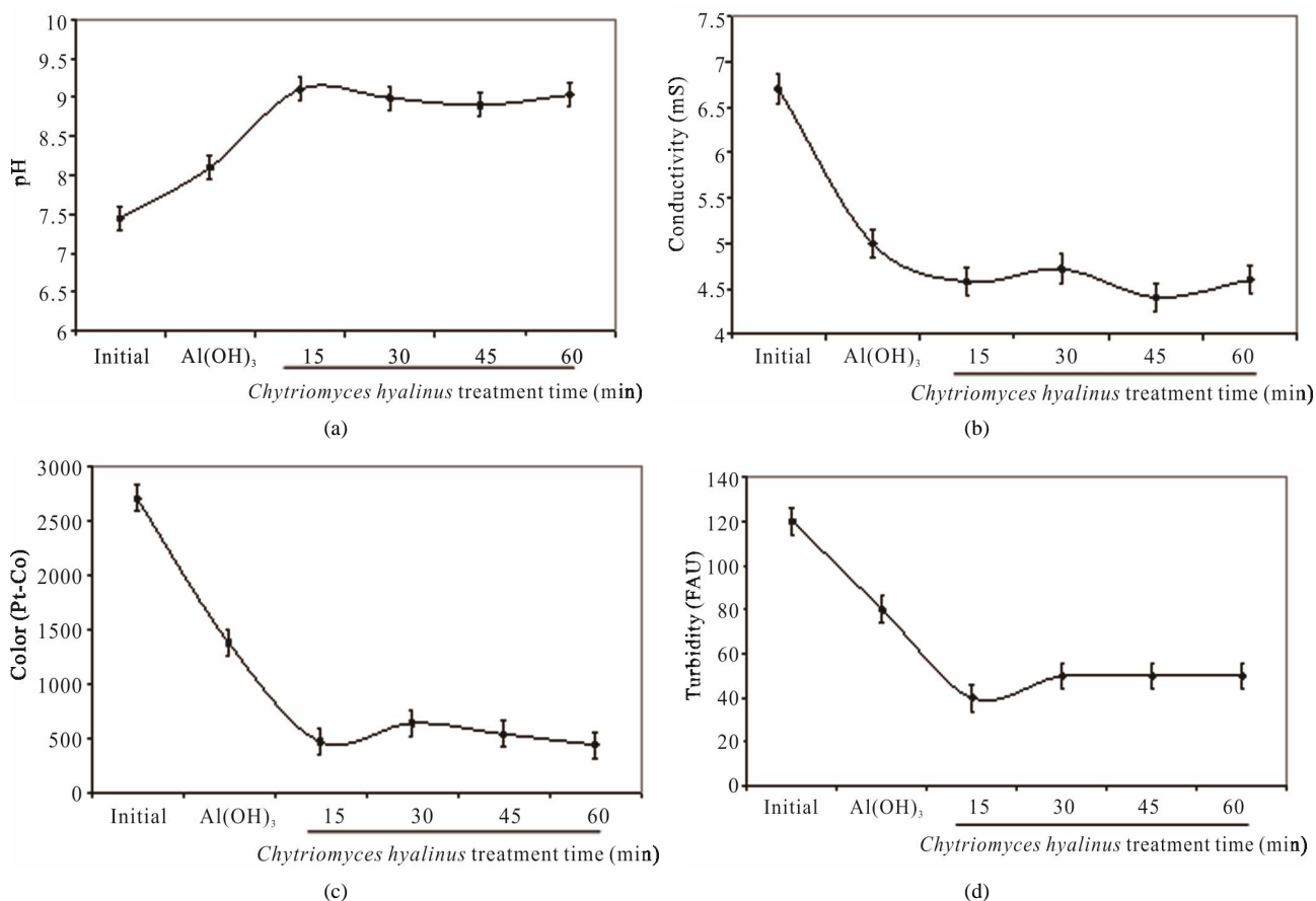
Figure 2. (a) pH; (b) Conductivity; (c) Color and (d) Turbidity during the electrochemical- Chytriomycetes hyalinus treatment.
