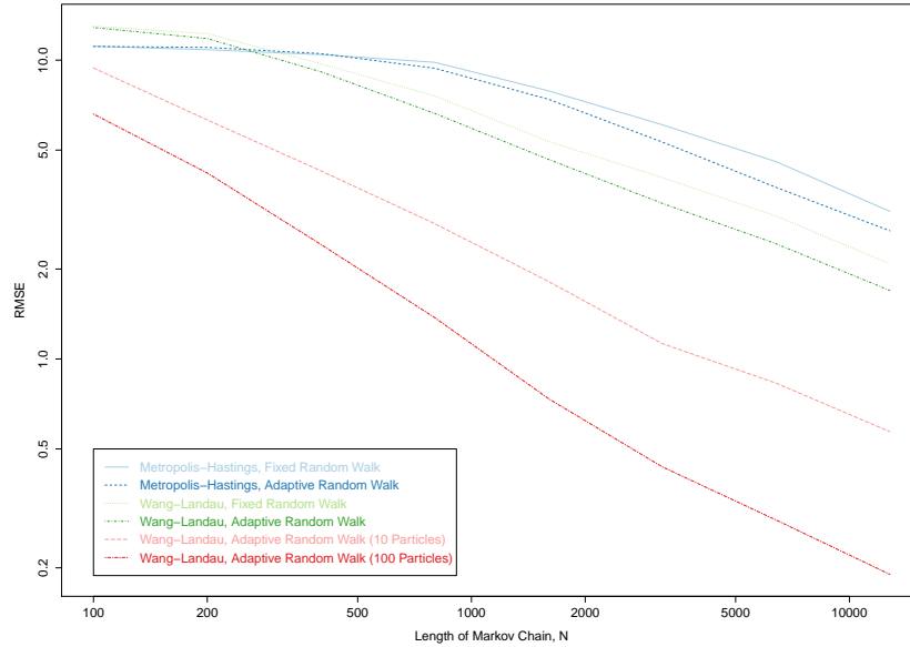
Fig. 2 RMSE for estimating the mean in the bimodal density for various simulated tempering configurations with and without adaptive proposals.
