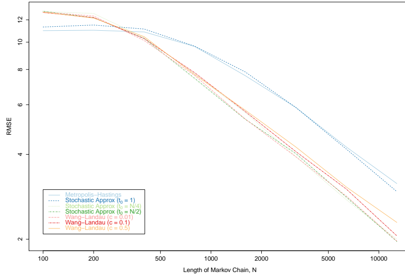
Fig. 1 RMSE for estimating the mean in the bimodal density for various simulated tempering configurations. We see that Wang-Landau (provided c is small) and stochastic approximation with deterministic step size decreases (provided t_0 is large) both perform well.
