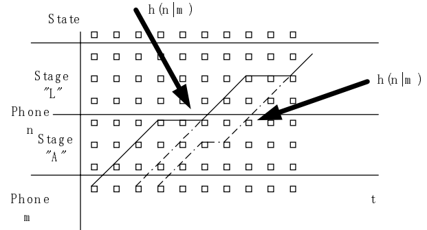
Figure 1: The illustration of the algorithm of the SLA 4. PRUNING STRATEGY BASED ON THE RANK OF LANGUAGE MODEL PROBABILITY
