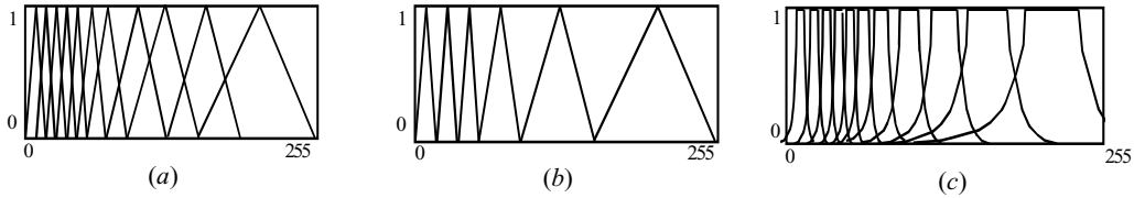
FIGURE 1. THE BAND-PASS FILTERS USED IN MFCC CALCULATION (horizontal axis: DFT frequency sampling point)
