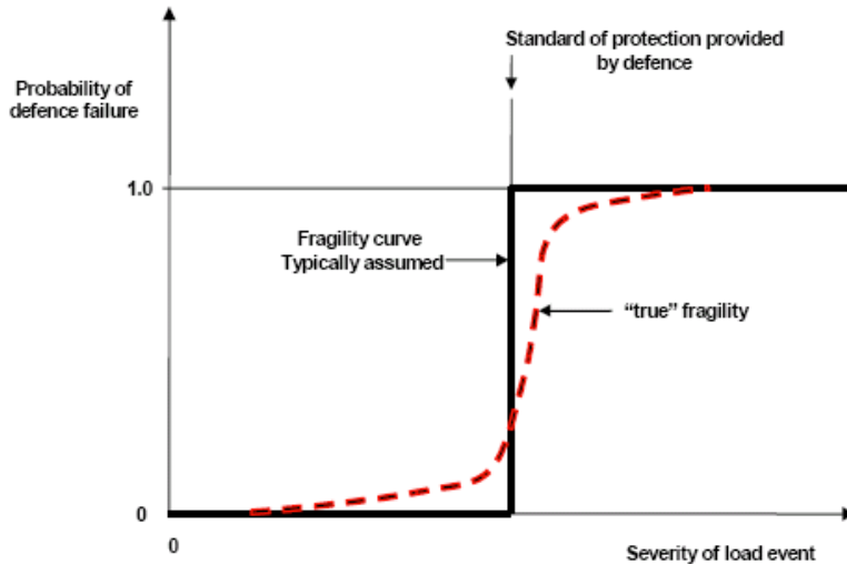
Figure 2: Example of a simplified and “true” generic fragility curve for flood defences
