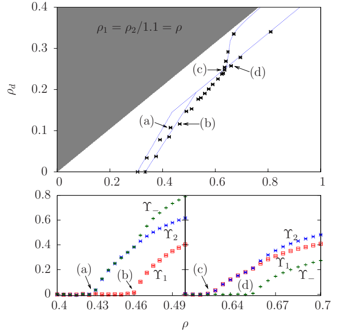
FIG. 6: (Color online) Phase diagram and a set of helicity moduli for the model Eq. (22), for \alpha = 1.1 . The shaded region illustrates the forbidden parameter regime \rho_d > \rho_1 \rho_2 / (\rho_1 + \rho_2) . The helicity moduli are \Upsilon_1, \Upsilon_2 , and \Upsilon_- . The left most helicity moduli are measured for a drag \rho_d = 0.25\rho , while the rightmost are \rho_d = 0.39\rho .
