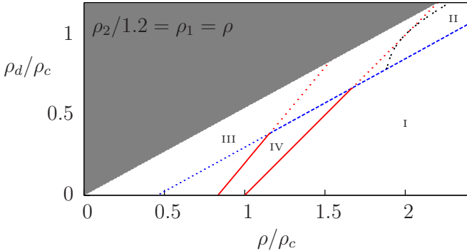
FIG. 2: (Color online) Schematic phase diagram with regions I, II, III, and IV for the model in Eqs. (1) and (13) with \rho_2 = \alpha\rho_1 > \rho_1 = \rho . For the purposes of illustration, we have taken \alpha = 1.2 . The gray shaded area is the forbidden parameter regime \rho_d > \alpha\rho/(1 + \alpha) . The lines separating the various regions are obtained as follows: a) Solid (red) lines : Proliferation of (0, 1) -vortices from an ordered background, along the line \rho_d = \alpha\rho - \rho_c , as well as proliferation of (0, 1) -vortices from an ordered background, along the line \rho_d = \rho - \rho_c . b) Dashed (blue) line : Proliferation of (1, -1) -vortices from an ordered background, along the line \rho_d = (1 + \alpha)\rho/4 - \rho_c/4 . c) Dashed-dotted (black) line : Line of proliferation of individual vortices (1, 0) or (0, 1) in a background of proliferated vortices (1, -1) , given by Eq. 16. When we cross this line from right to left, passing from region II to III, the stiffness of the clapping mode \theta_1 + \theta_2 is destroyed by the proliferation of individual vortices.
