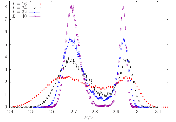
FIG. 5: (Color online) The energy histograms for (\rho, \rho_d) \approx (0.60, 0.20) , with \alpha = 1 , i.e. in the preemptive region. A clear double peak structure is seen to develop, an indication of a first order transition. The areas under the histograms are normalized to 1.
