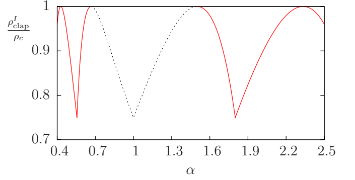
FIG. 3: (Color online) Plot of \rho_{\text{clap}}(\rho_I, \rho_{dI}, \alpha)/\rho_c as a function of \alpha . Note that the system is symmetric around \alpha = 1 . The dashed (black) line in the above figure shows that the remaining stiffness of the clapping mode (in the background of proliferated composite (1, -1) -vortices) is less than the critical coupling for vortex-loop proliferation in a parameter regime 2/3 < \alpha < 3/2 . This is the parameter regime where it is correct to limit oneself to the sector where the composite proliferated background vortices are of the type (1, -1) . For \alpha < 2/3 , the composite proliferated background vortices are of type (-n, 1) , while for \alpha > 3/2 , the composite proliferated background vortices are of type (1, -n) . The fact that \rho_{\text{clap}}(\rho_I, \rho_{dI}, \alpha) < \rho_c indicates that we are in a parameter regime where the full restoration of U(1) \times U(1) -symmetry proceeds from a preemptive vortex-loop proliferation phase transition, as explained in the text. The solid (red) line in the above figure shows \rho_{\text{clap}}(\rho_I, \rho_{dI}, \alpha) for \alpha < 2/3 in a regime where (2, -1) -vortices trigger preemptive proliferation of all topological defects and \alpha > 3/2 where (1, -2) -vortices initiate the phase transition into fully symmetric state.
