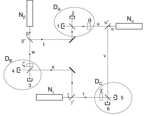
FIG. 2: Each of 3 condensates is split in 2 parts, which then enter interferometers in 3 remote places D_A , D_B and D_C ; the quantum results show GHZ contradictions with local realism.
