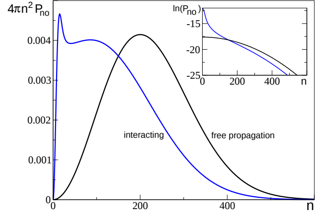
FIG. 1: (Color online). Form of 4\pi n^2 P_{n0}(t) after time t such that z = 2\Delta_o t \gg R^2 , calculated from Eq.(11) with z = 2000 and R = 10 for the three-dimensional walker. The inset for \ln P_{n0} shows the asymptotic decay.
