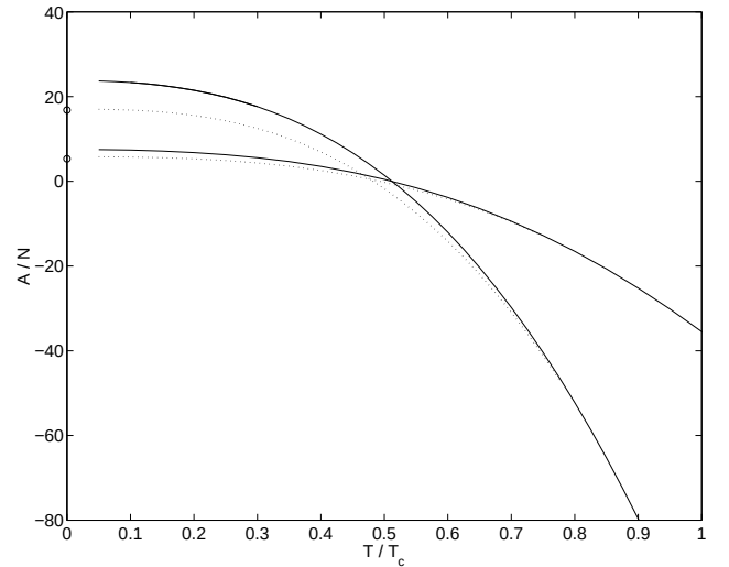
FIG. 3: Free energies per particle for the condensed (dashed line) and uncondensed (full line) solutions. The curves with higher value at T = 0 correspond to N = 10^4 atoms, while those with the lower value at T = 0 correspond to N = 10^3 . The coupling constant is \tilde{\gamma} = 0.1 in both cases. The open circles on the vertical axis are the Thomas-Fermi predictions given by Eq. (22) for T = 0 . The free energies seem to be converging in the high-temperature limit; the low-temperature limit, on the other hand, shows the discrepancy that results from restricting condensate fluctuations (see discussion after Eq. (23)). Note that T_c , the transition temperature for the ideal 2D trapped gas, depends on N ; thus the x axis for each N represents a different actual temperature.
