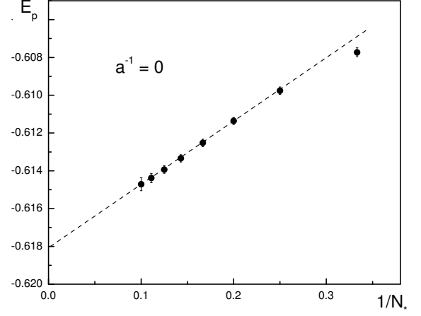
FIG. 5: The polaron energy (at the unitarity point a^{-1} = 0 ) as a function of truncation parameter N_* for the advance summation technique. The asymptotic behavior at 1/N_* \rightarrow 0 is perfectly fit by a straight line.
