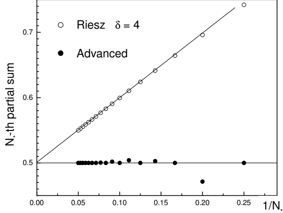
FIG. 4: Summing the Grandi series, 1 - 1 + 1 - 1 + \dots = 1/2 , by Riesz method and by the advanced method described in the text. The solid lines are to guide an eye.
