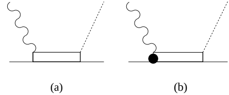
FIG. 1. Feynman diagrams for the \bar{\gamma}N \rightarrow \Delta \rightarrow \pi N process. The dark circle indicates a parity violating coupling.
