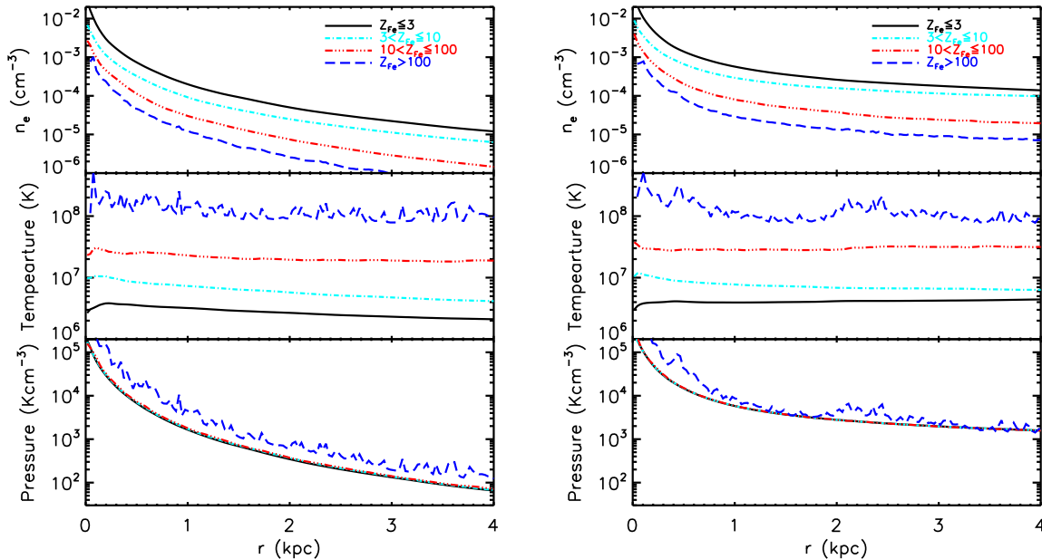
Fig. 4.— Average radial electron number density, temperature, and pressure profiles for the supersonic (left panel) and subsonic (right panel) cases. The profiles are plotted separately for the gas components with different iron abundances: Z_{\text{Fe}} \leq 3 (solid black line), 3 < Z_{\text{Fe}} \leq 10 (dash-dot cyan line), 10 < Z_{\text{Fe}} \leq 100 (dash-three-dots red line), and Z_{\text{Fe}} > 100 (long-dash blue line).
