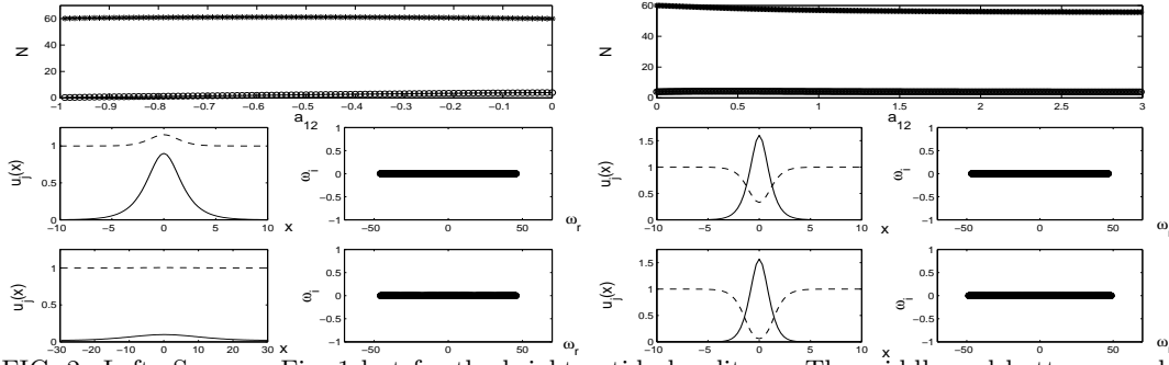
FIG. 2. Left: Same as Fig. 1 but for the bright-antidark solitons. The middle and bottom panels are for a_{12} = -0.5 and a_{12} = -0.99 , respectively. Right: The branch of coupled bright-gray solitons. The middle and bottom panels are for a_{12} = 0.2 and 0.5 , respectively.
