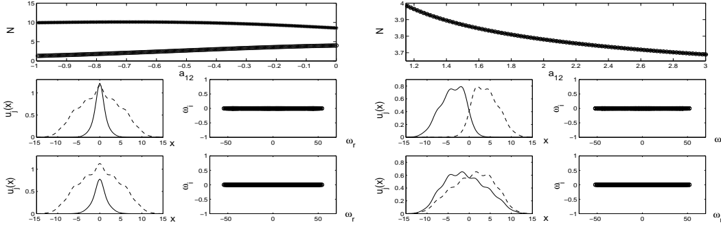
FIG. 3. Left: The bright-antidark branch (the middle and bottom panel are for a_{12} = -0.5 and -1 , respectively) in the presence of the potential V(x) = 0.01x^2 + 0.5\sin^2(x) , see Eq. (2). Right: The same for the domain-wall solutions (the middle and bottom panels are for a_{12} = 3 and 2 , respectively).
