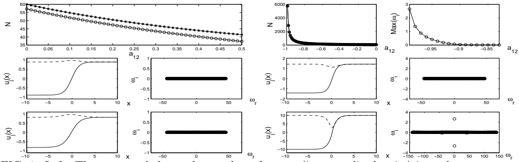
FIG. 1. Left: The top panel shows the number of atoms (in normalized units) in each component (circles and stars) of the dark-antidark soliton. The middle and bottom left panels show the spatial profiles of this solution for a_{12} = 0.2 and a_{12} = 0.5 , while the right panels show the respective spectral planes ( \omega_r, \omega_i ) of the corresponding eigenfrequencies, as found from the linearized equations ( \omega_i = 0 implies linear stability). Right: The top panels show the number of atoms in each component of the dark-gray soliton and the instability growth versus a_{12} . The middle and bottom left panels show the spatial profiles of this solution for a_{12} = -0.5 and a_{12} = -0.99 , while the right panels show the respective spectral planes.
