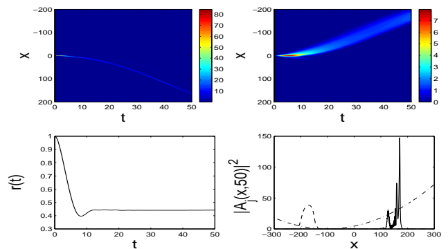
FIG. 3: The top left and right panels show space-time contour plots of the 1st and 2nd band wavefunctions respectively. The bottom left shows the temporal evolution of the tunneling rate r(t) , while the bottom right shows a snapshot of the solution at t = 50 . Solid line: |A_1|^2 ; dashed line: |A_2|^2 ; dash-dotted: parabolic potential.
