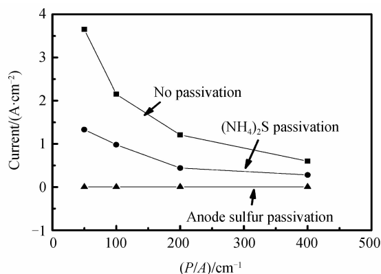
图 4 超晶格二极管漏电流密度与面积周长比 ( P/A ) 关系 Fig. 4 The relation between current density and P/A for different sized photodiodes
