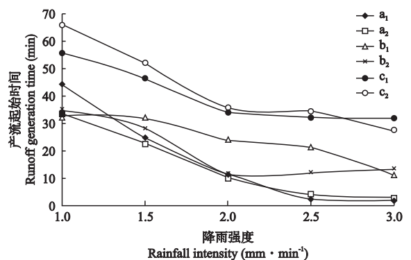
图 1 弃土弃渣体产流起始时间随降雨强度的变化 Fig. 1 Variation of runoff generation time with rainfall intensity for the residues.
